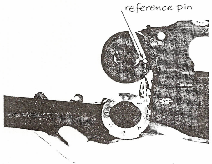
placing short and long eyepieces onto viewfinder
