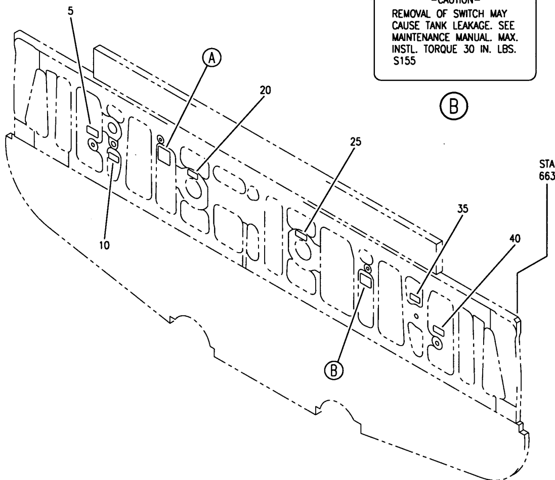
MARKING INSTL-SECT. 11 REAR SPAR FUEL SYS FIGURE 3
