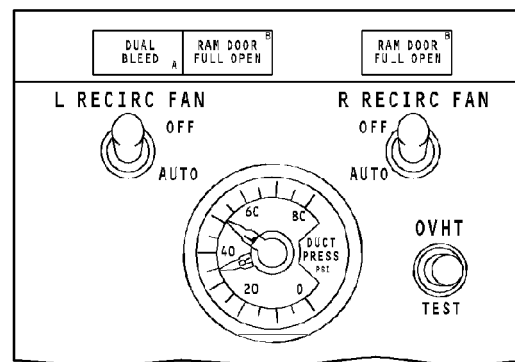
AIR CONDITIONING/BLEED AIR CONTROLS PANEL
