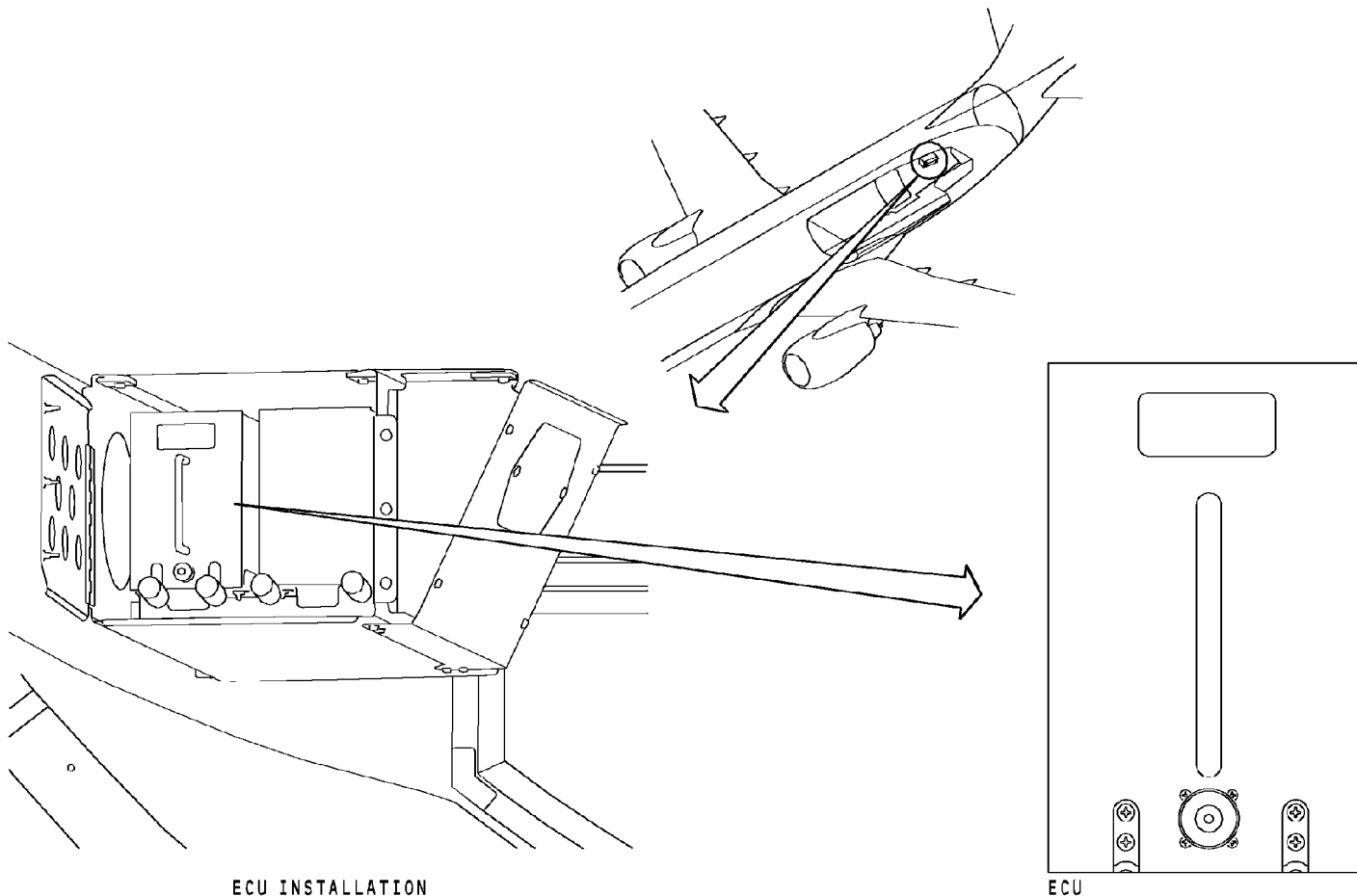
ECU INSTALLATION
