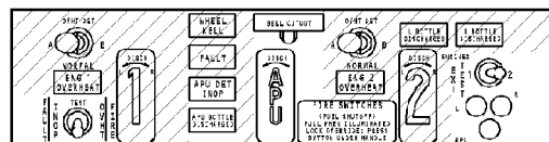
ENGINE AND APU FIRE CONTROL PANEL (P8)
