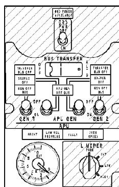
AC SYSTEM GENERATOR/ APU CONTROL PANEL (P5)
