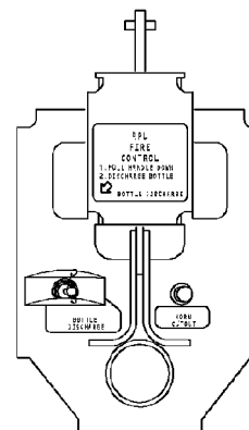
APU GROUND CONTROL PANEL (P28 RIGHT WHEEL WELL)
