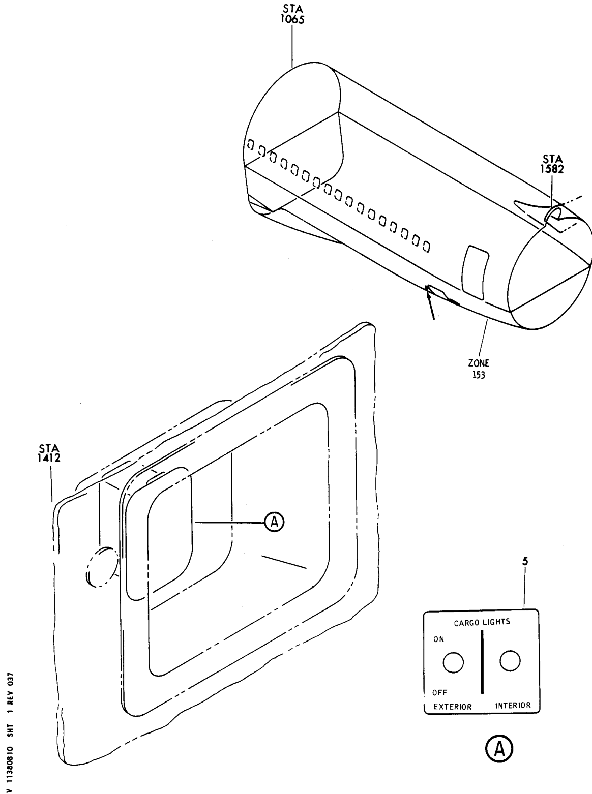
SWITCH INSTL-BULK CARGO LIGHTS (PLACARDS AND MARKINGS ONLY) FIGURE 10
