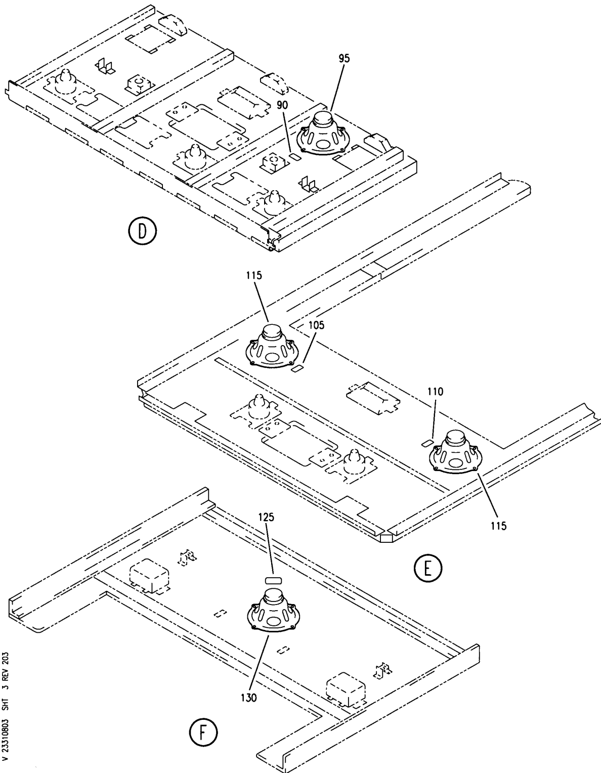
CEILING ASSY-MID CABIN LOWERED(SPEAKERS ONLY) FIGURE 3 (SHEET 3)
