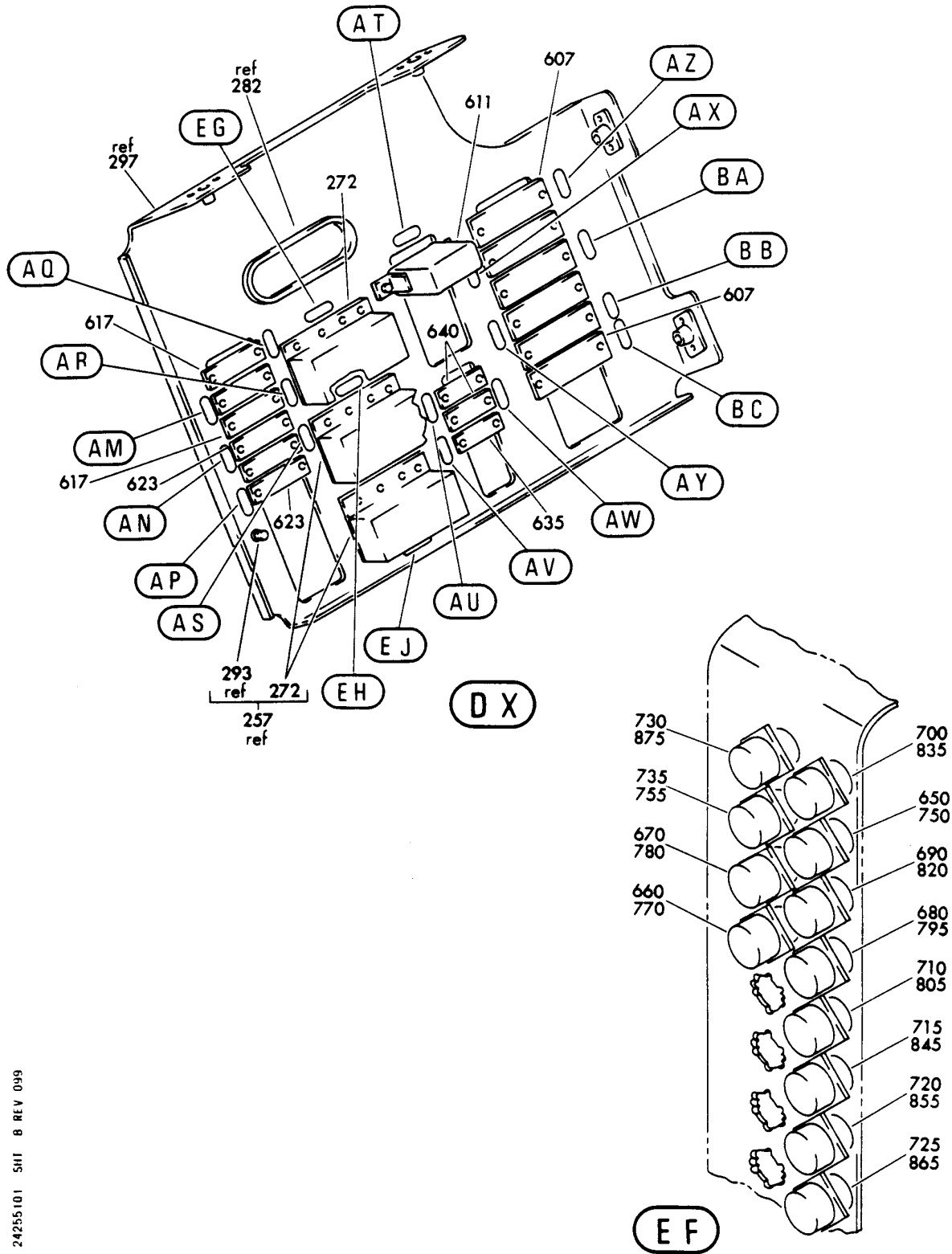
PANEL INSTL-P65 FIGURE 1 (SHEET 8)
