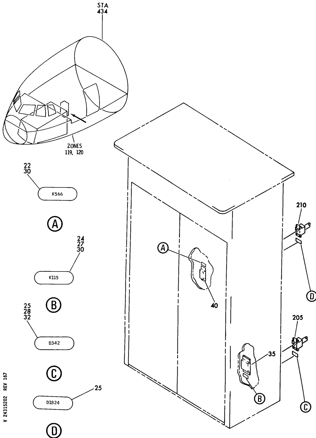
EQUIPMENT ASSY-P33 MISC ELEC PNL FWD (BATTERIES ONLY) FIGURE 2
