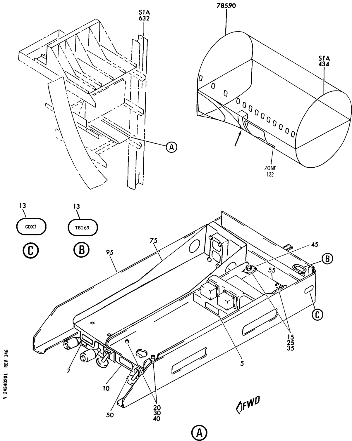
SHELF ASSY-ELECTRONICS EQUIP CTR E5-3 (MEDICAL OUTLETS INVERTER ONLY)
