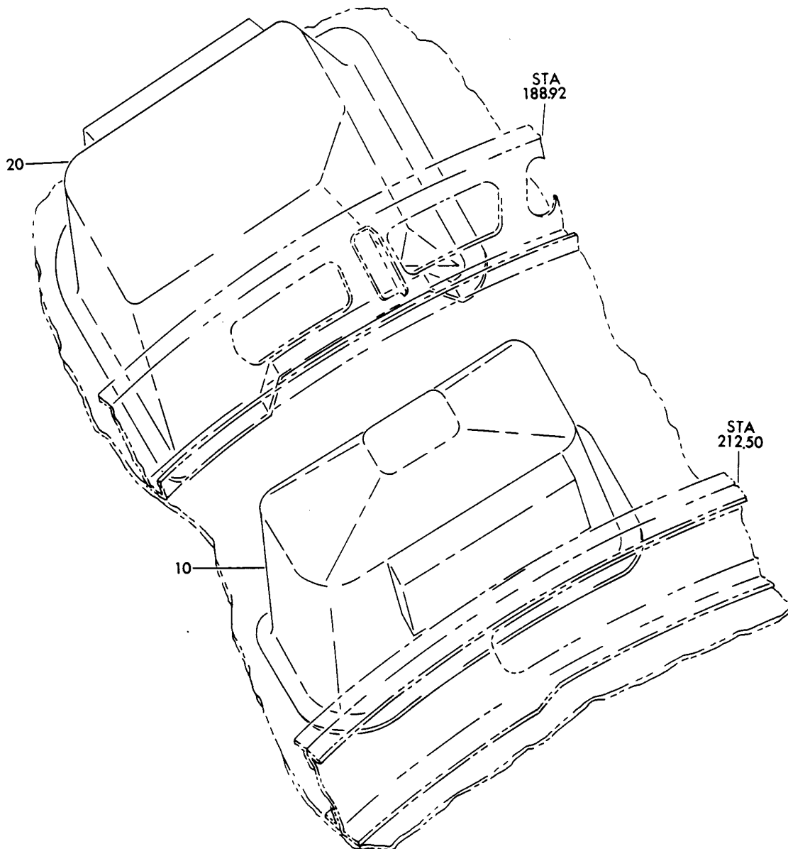
REVEAL INSTL-WINDOW TRACKS FLEXIBLE FIGURE 1
