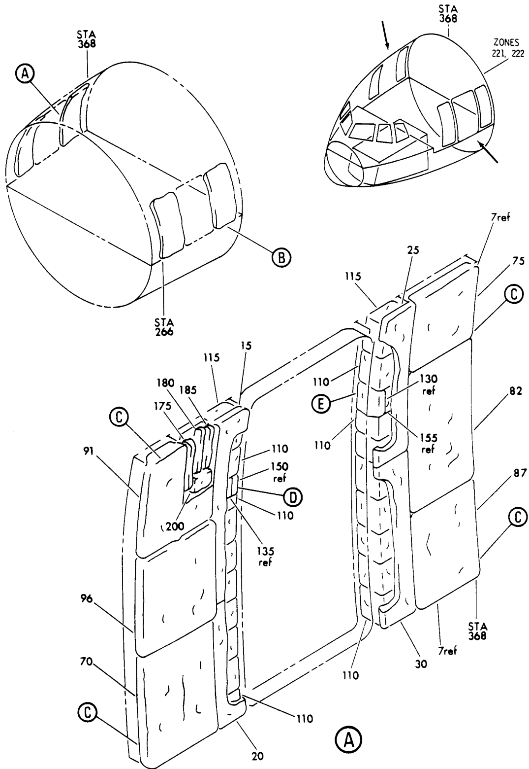
INSULATION INSTL-SECT. 41 PASS. CAB. DOORWAYS FIGURE 20 (SHEET 1)
