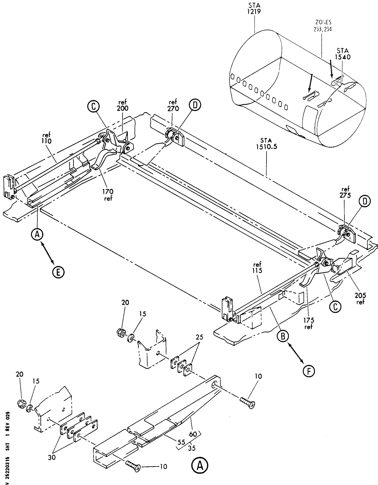
MECHANISM INSTL-MOVABLE CLG AFT FIGURE 15 (SHEET 1)
