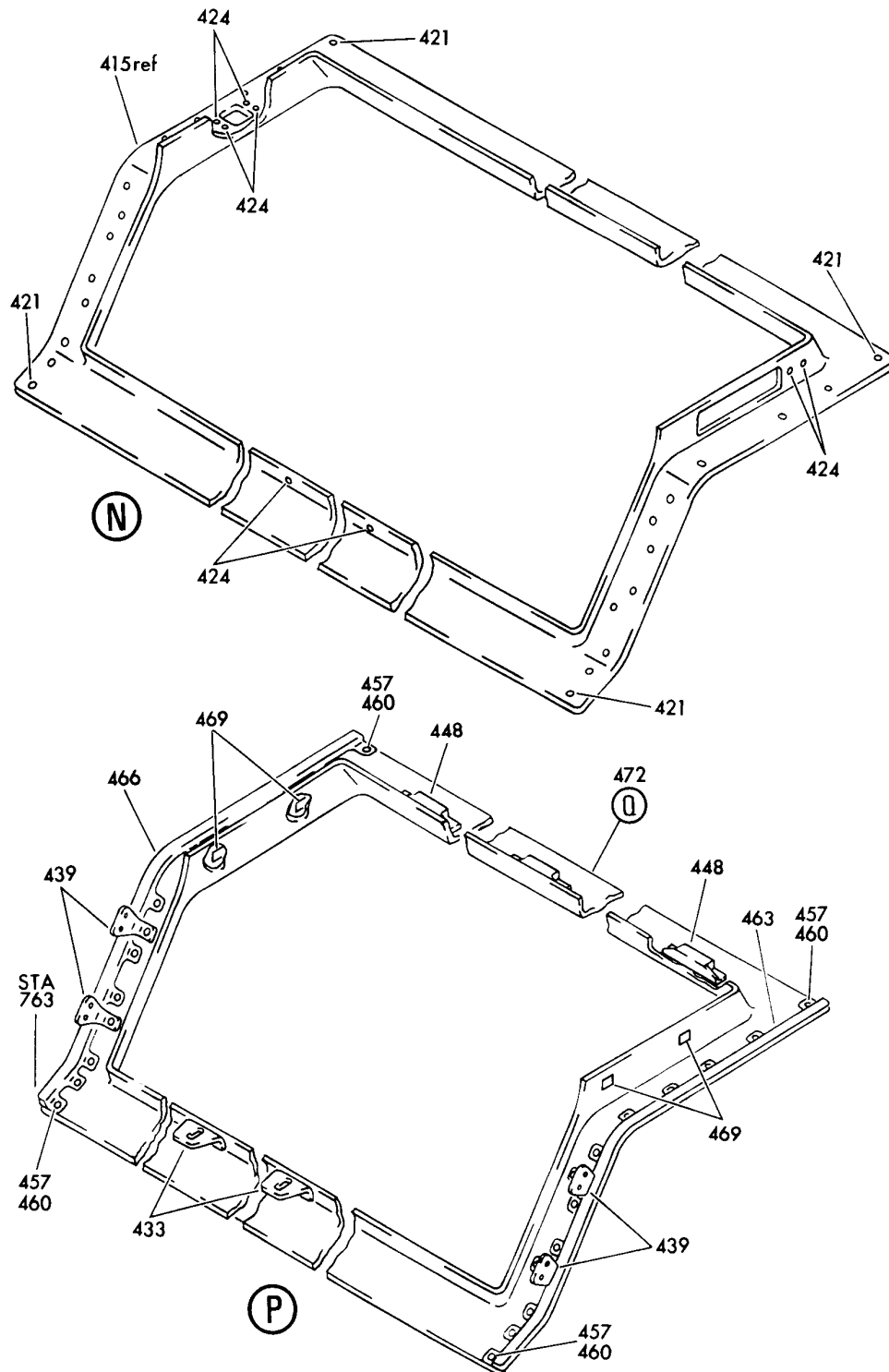
FRAME ASSY-CLG (EQUIPMENT/ FURNISHINGS ONLY) FIGURE 14S (SHEET 8)
