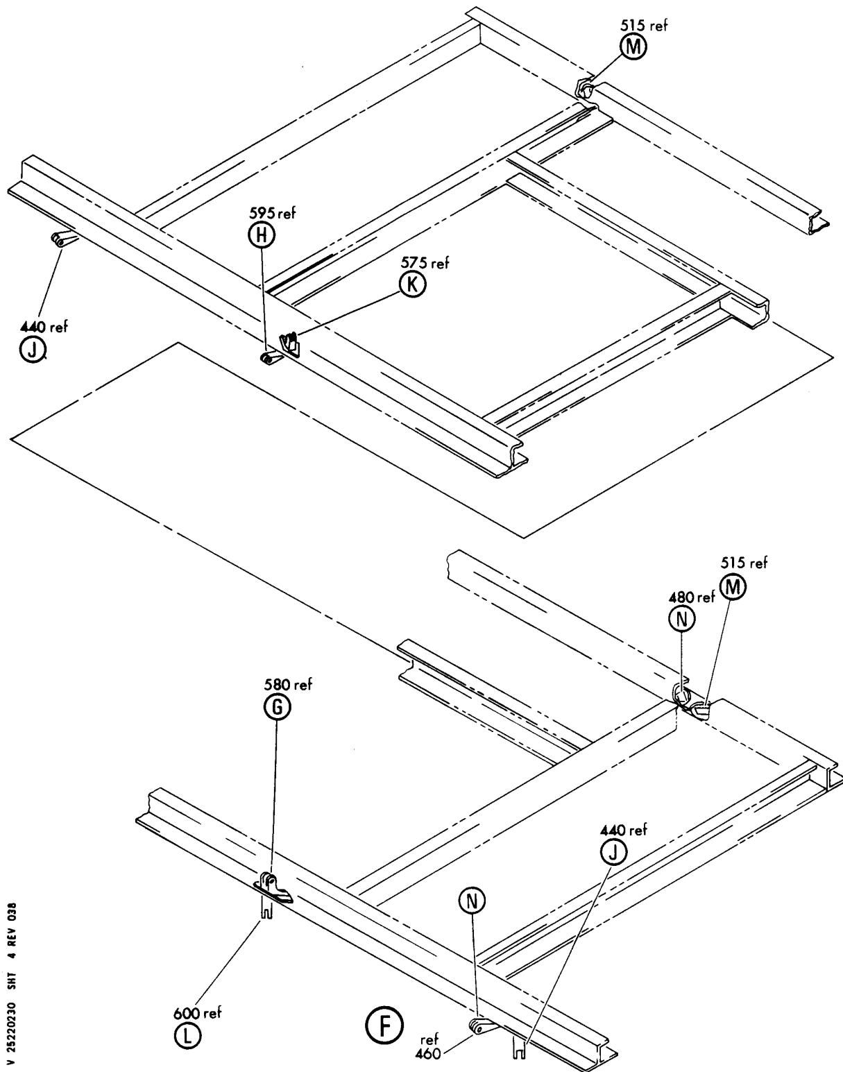
SUPPORT INSTL-AFT OVER ENTRY LOWERED CLG FIGURE 30 (SHEET 4)
