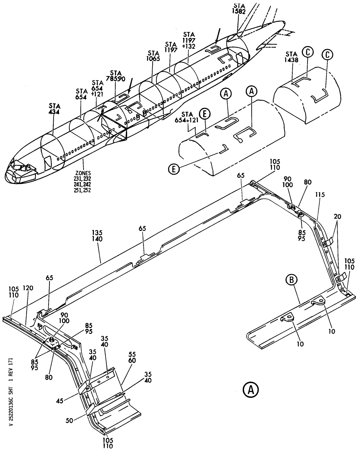
FRAME ASSY-CLG (EQUIPMENT/ FURNISHINGS ONLY) FIGURE 36C (SHEET 1)
