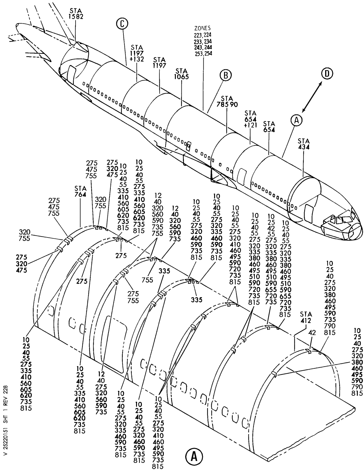
BRACKET INSTL-SCULPTURED CLG FIGURE 51 (SHEET 1)
