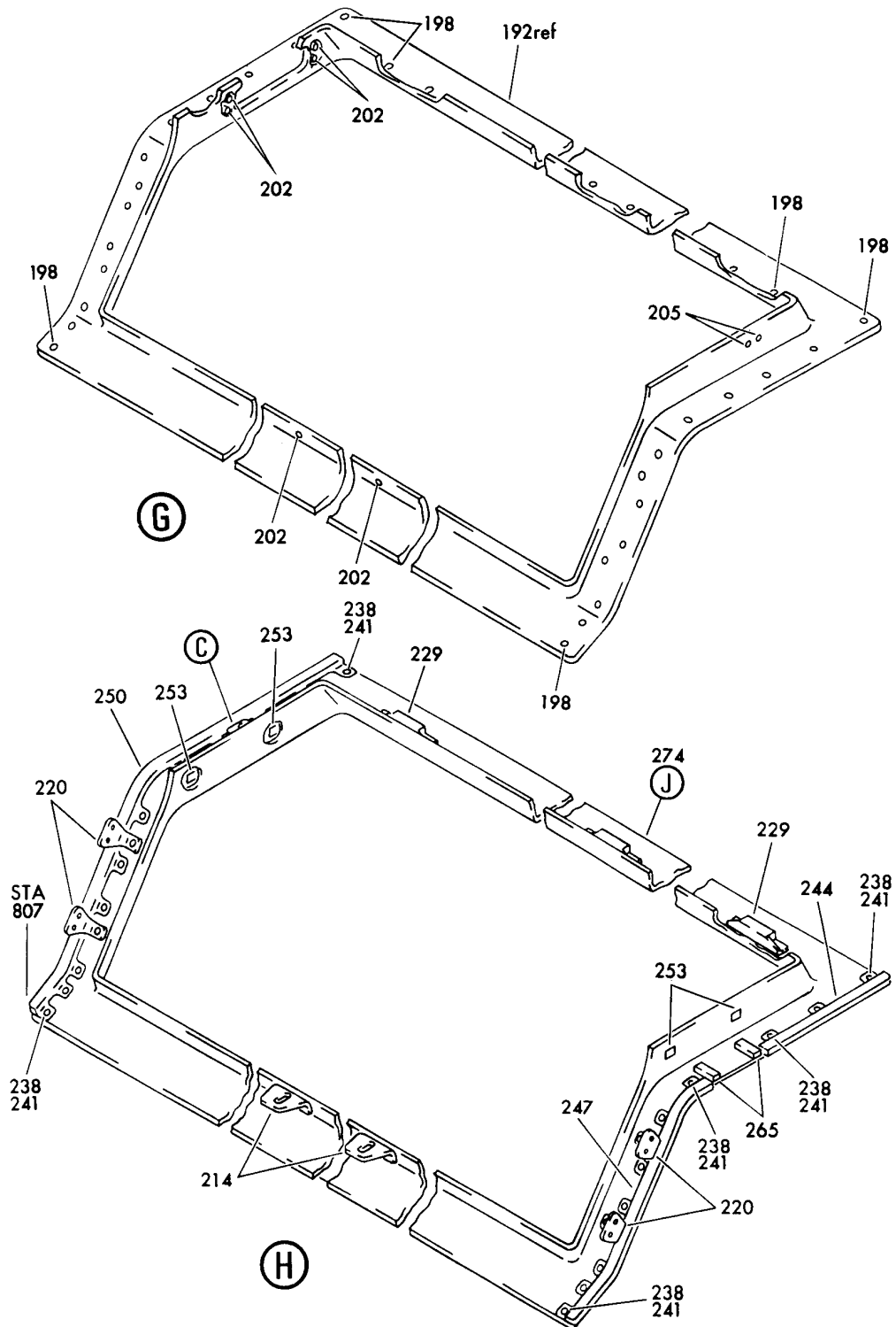
FRAME ASSY-CLG (EQUIPMENT/ FURNISHINGS ONLY) FIGURE 14S (SHEET 5)
