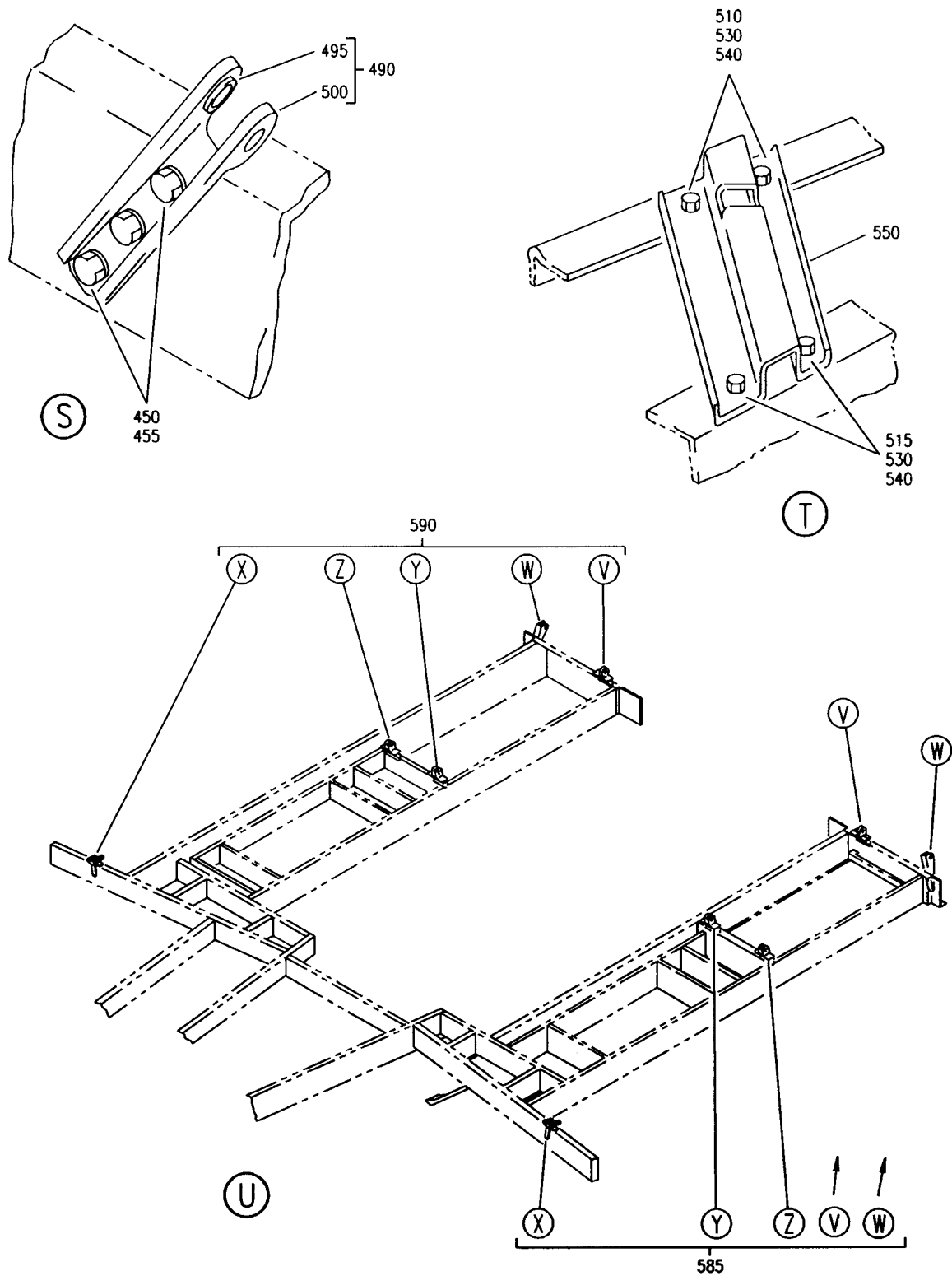
SUPPORT INSTL-OVER ENTRY LOWERED CLG FWD FIGURE 15 (SHEET 7)
