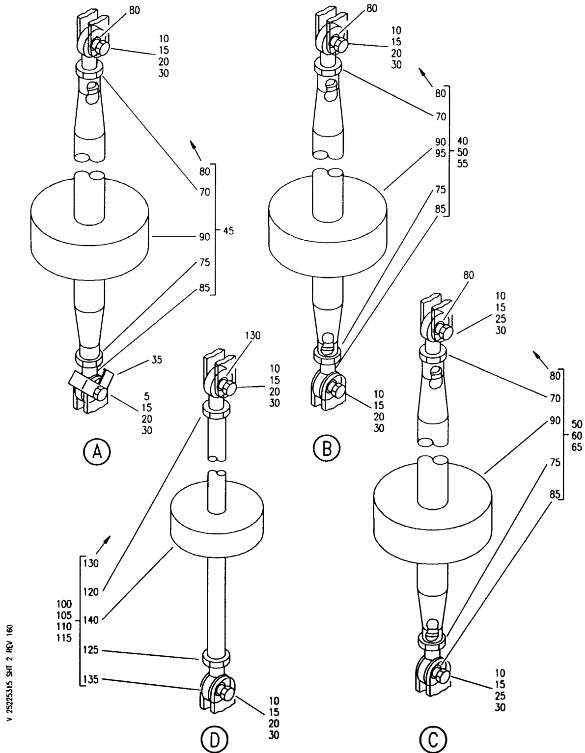
SUPPORT INSTL-OVER ENTRY LOWERED CLG FWD FIGURE 15 (SHEET 2)
