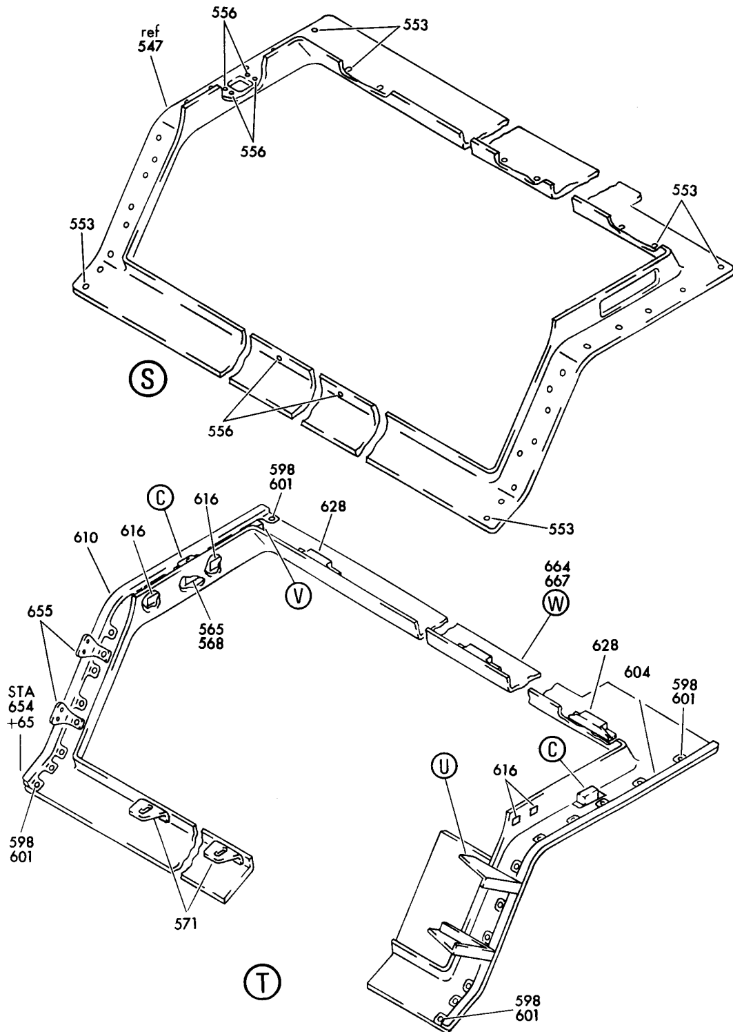
FRAME ASSY-CLG (EQUIPMENT/ FURNISHINGS ONLY) FIGURE 14S (SHEET 10)
