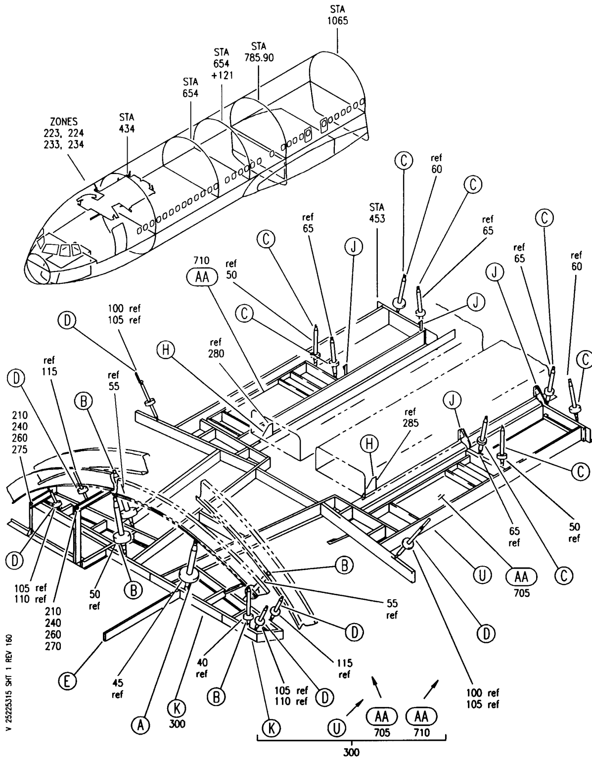
SUPPORT INSTL-OVER ENTRY LOWERED CLG FWD FIGURE 15 (SHEET 1)
