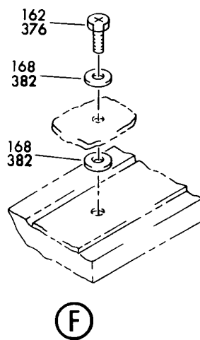
FRAME ASSY-CLG (EQUIPMENT/ FURNISHINGS ONLY) FIGURE 14S (SHEET 4)
