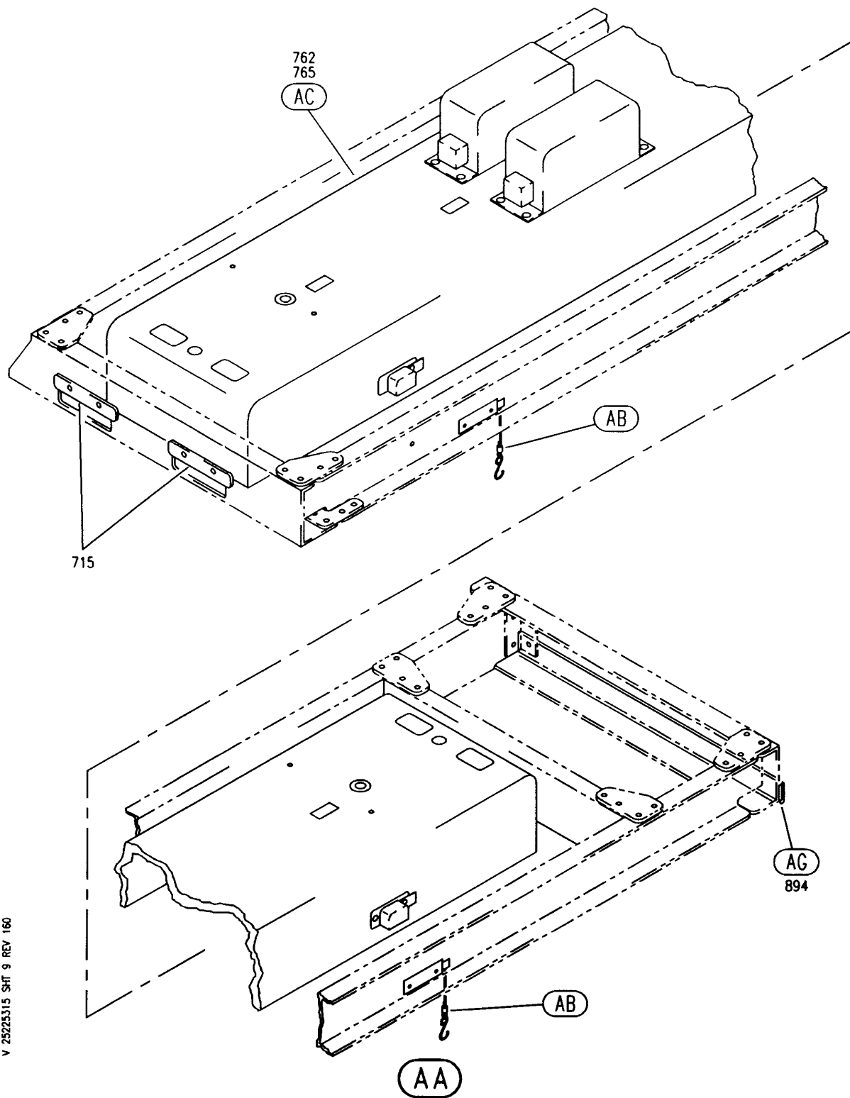
SUPPORT INSTL-OVER ENTRY LOWERED CLG FWD FIGURE 15 (SHEET 9)
