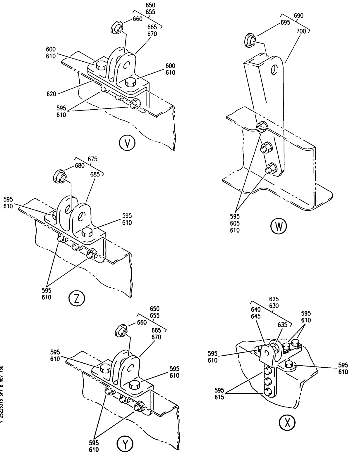
SUPPORT INSTL-OVER ENTRY LOWERED CLG FWD FIGURE 15 (SHEET 8)
