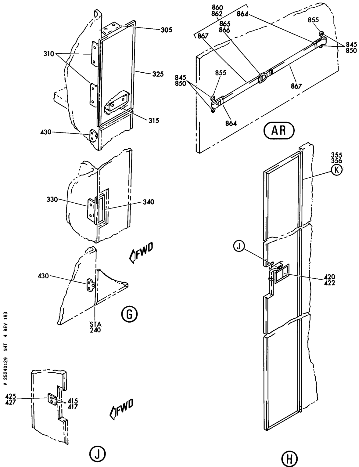
CLOSET INSTL-STA 240.5 FIGURE 29 (SHEET 4)
