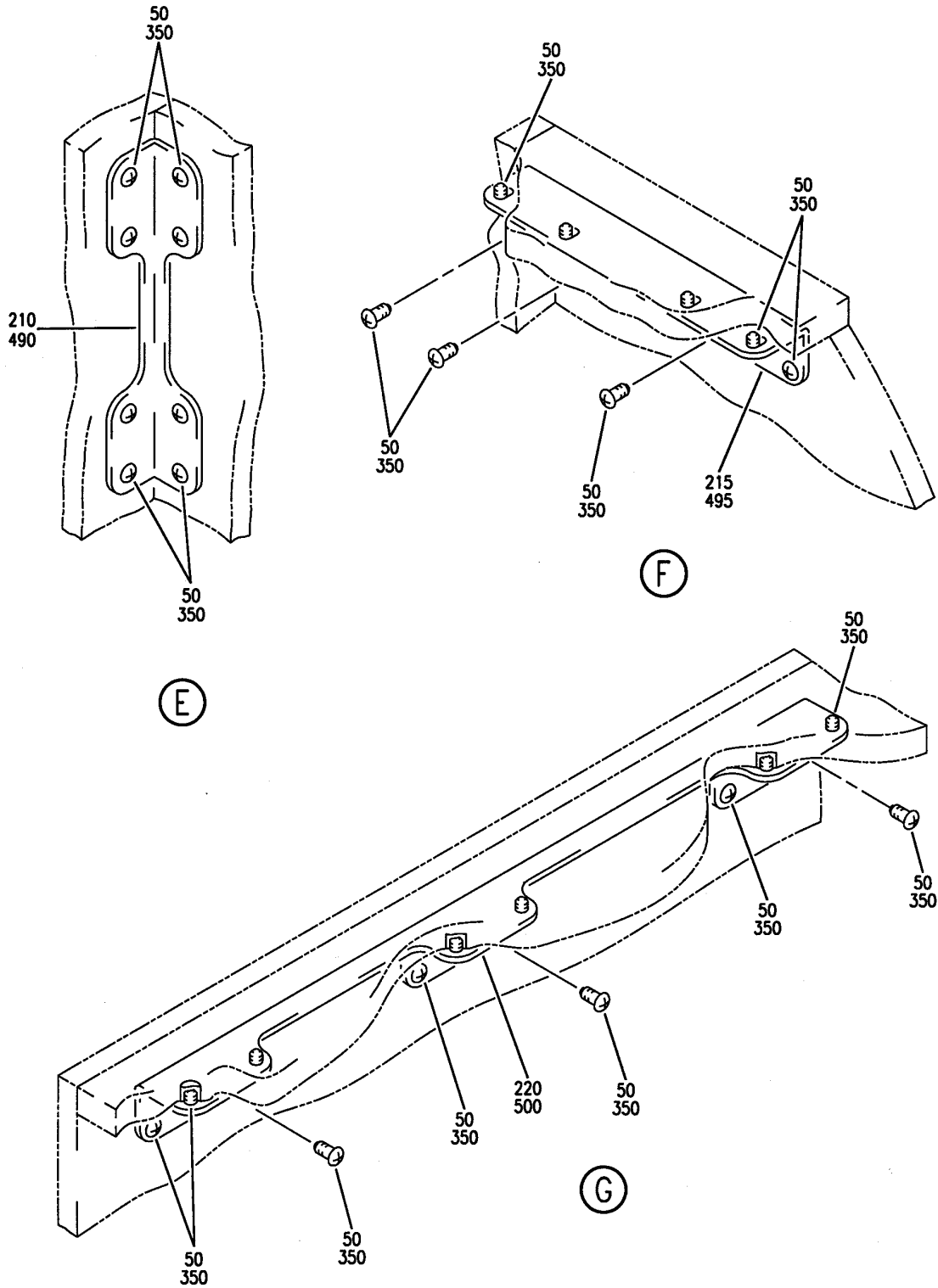
BIN ASSY-CTR OVERHEAD STOWAGE FIGURE 37C (SHEET 4)
