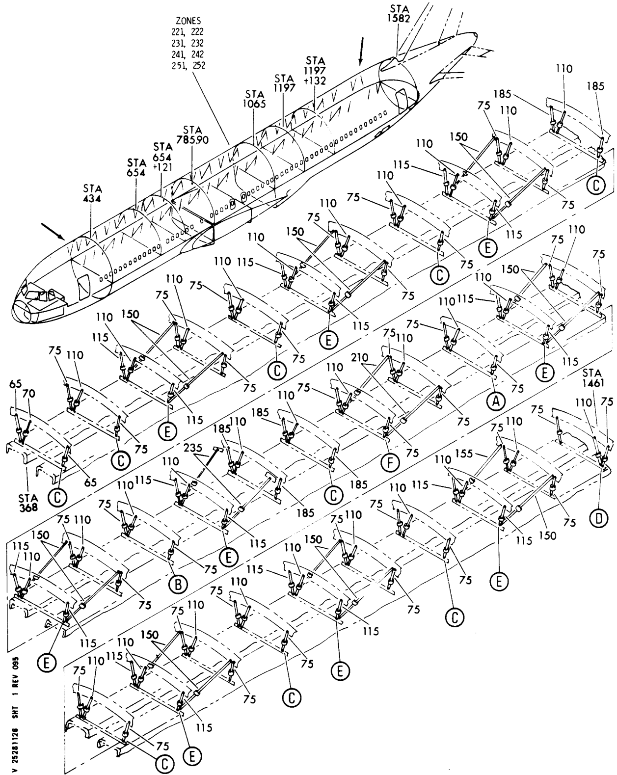
STRUT INSTL-CTR STOWAGE SPT FIGURE 26 (SHEET 1)
