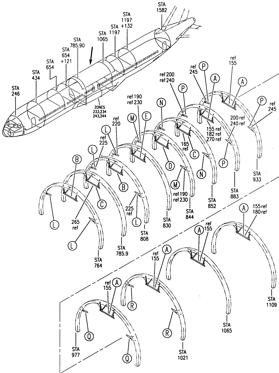
JUMPER INSTL-STOWAGE BINS MULTI-SECT. UPPER STA 764-STA 1109 FIGURE 2A (SHEET 1)
