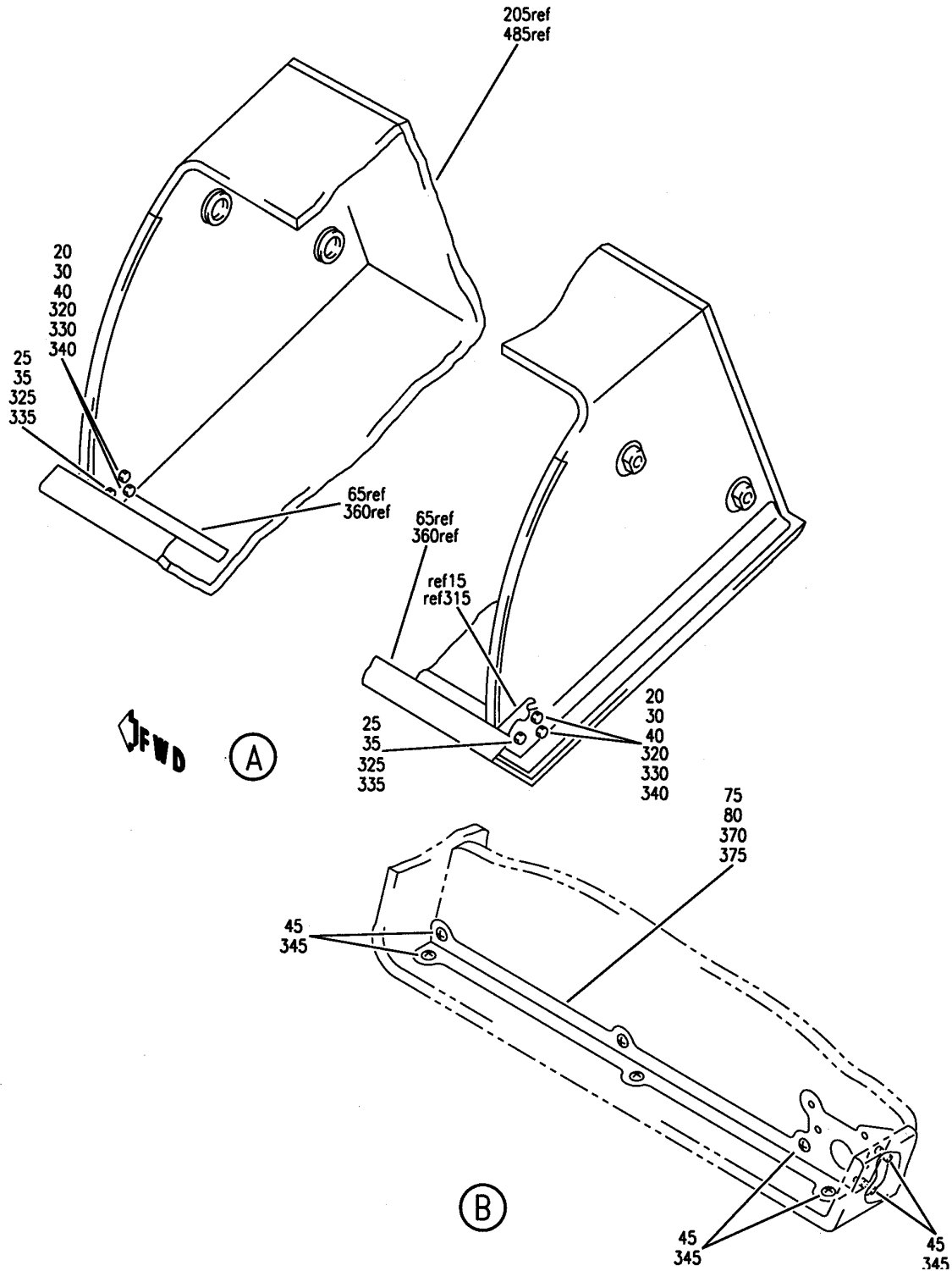
BIN ASSY-CTR OVERHEAD STOWAGE FIGURE 37C (SHEET 2)
