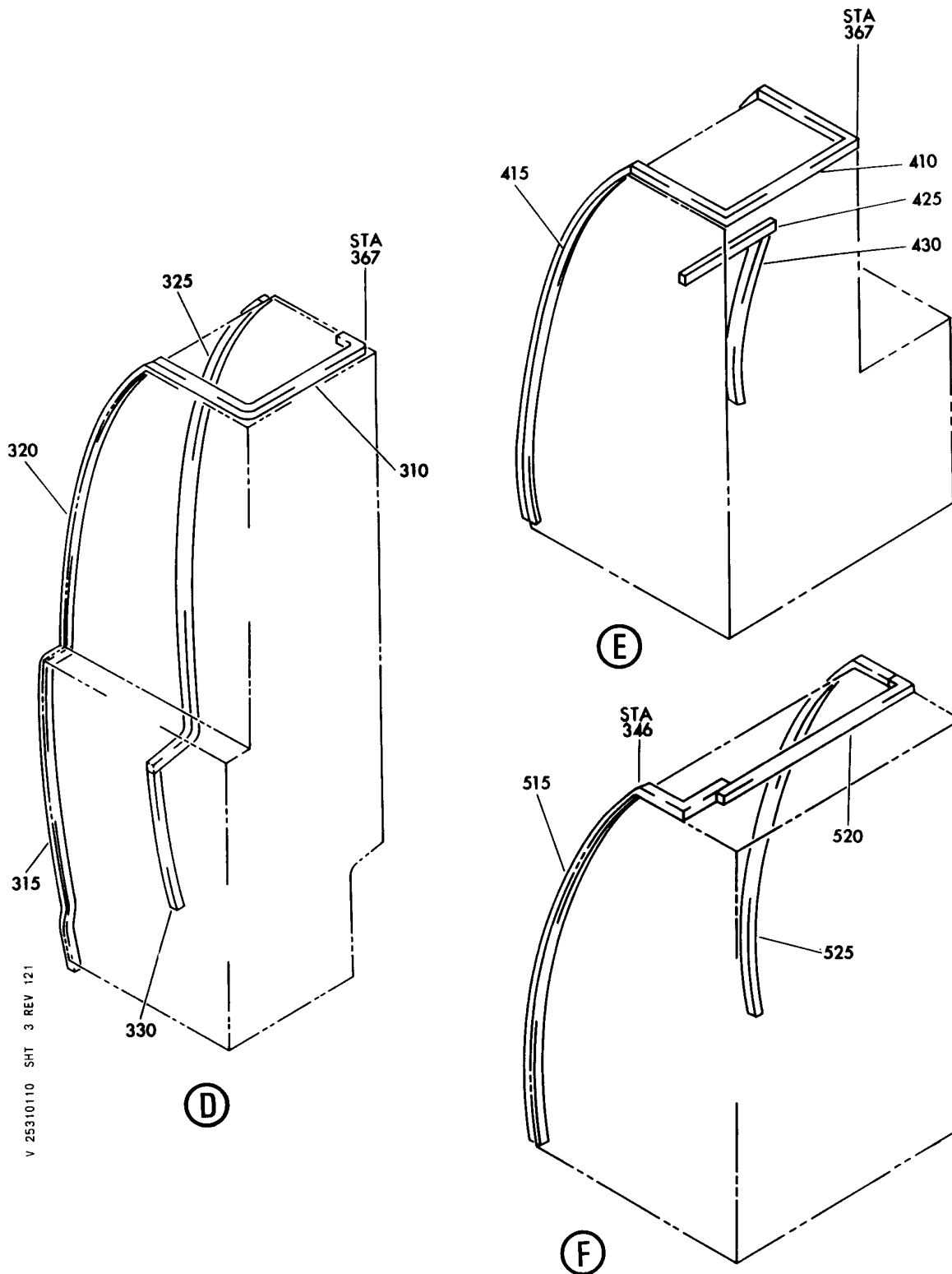
TRIM INSTL-FWD GALLEY FIGURE 10 (SHEET 3)
