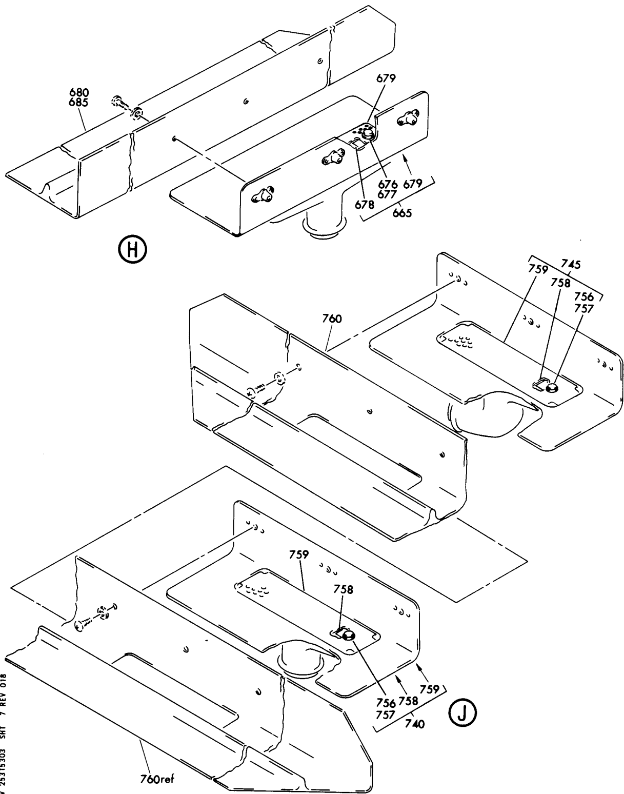
THRESHOLD, RETAINER, GUTTER AND BRIDGE-GALLEY FLOOR FIGURE 3 (SHEET 7)
