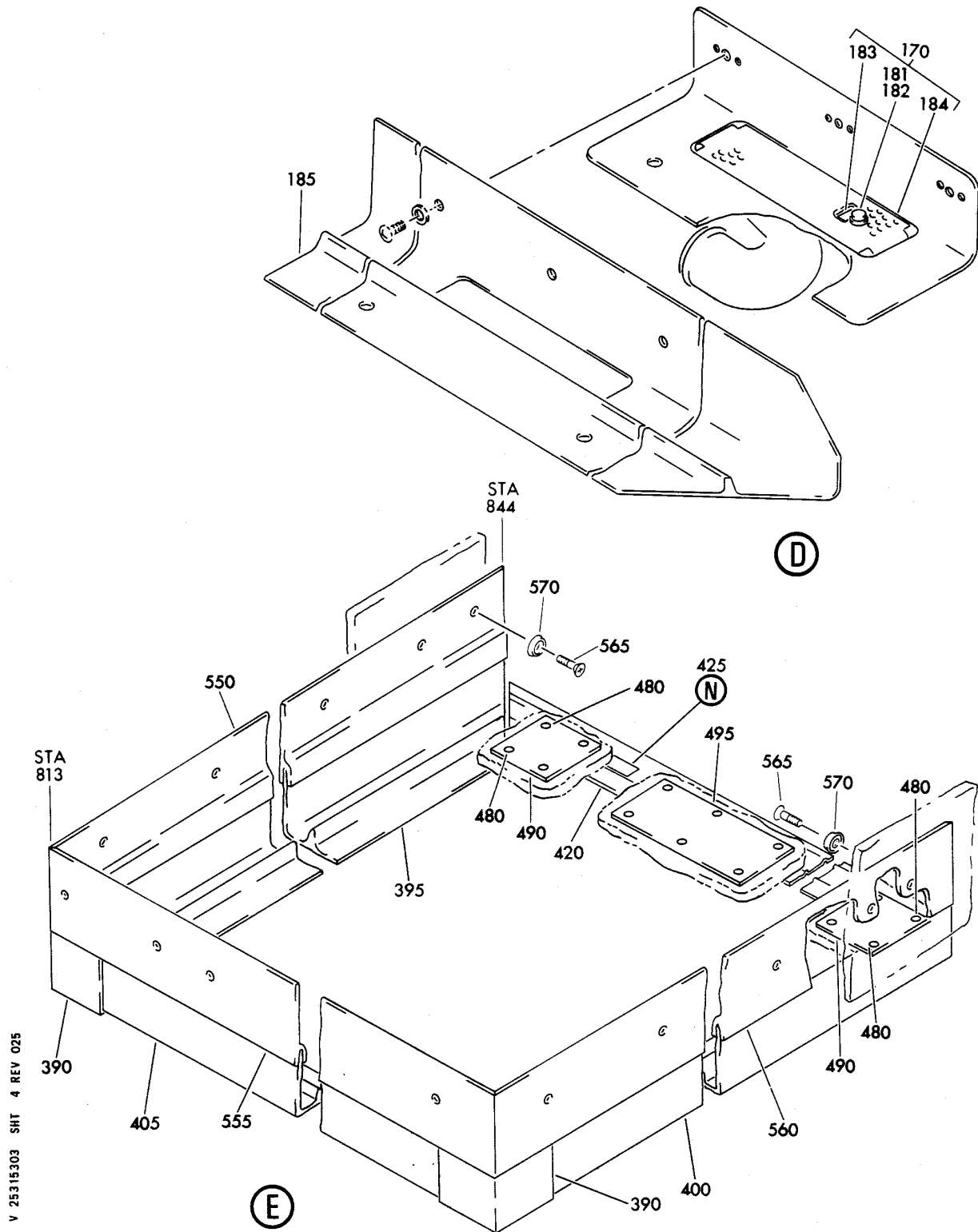
THRESHOLD, RETAINER, GUTTER AND BRIDGE-GALLEY FLOOR FIGURE 3 (SHEET 4)
