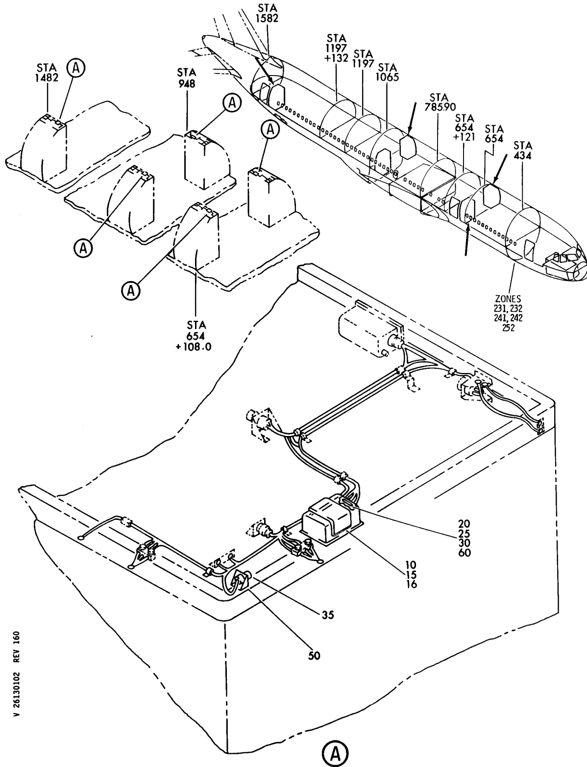
SMOKE DETECTOR INSTL-LAV FIGURE 2
