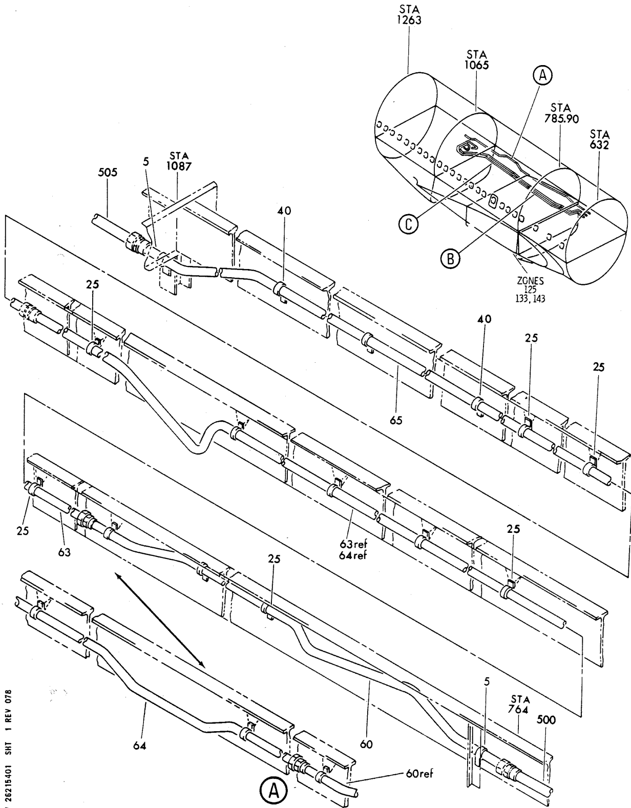
TUBING INSTL-WING/WHEEL WELL FIRE EXT FIGURE 1 (SHEET 1)
