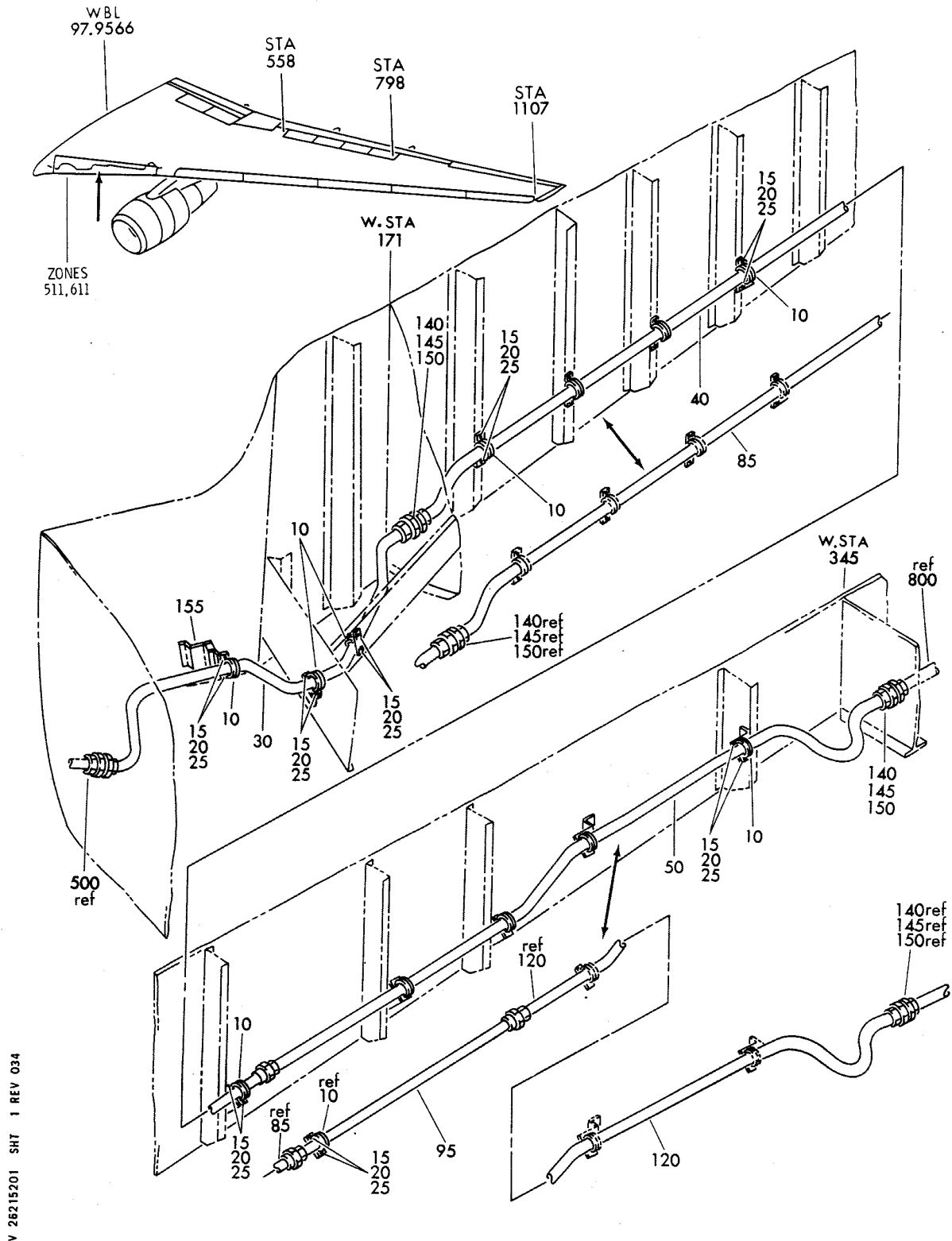
PLUMBING INSTL-ENG FIRE EXT SYS WING LE FIGURE 1
