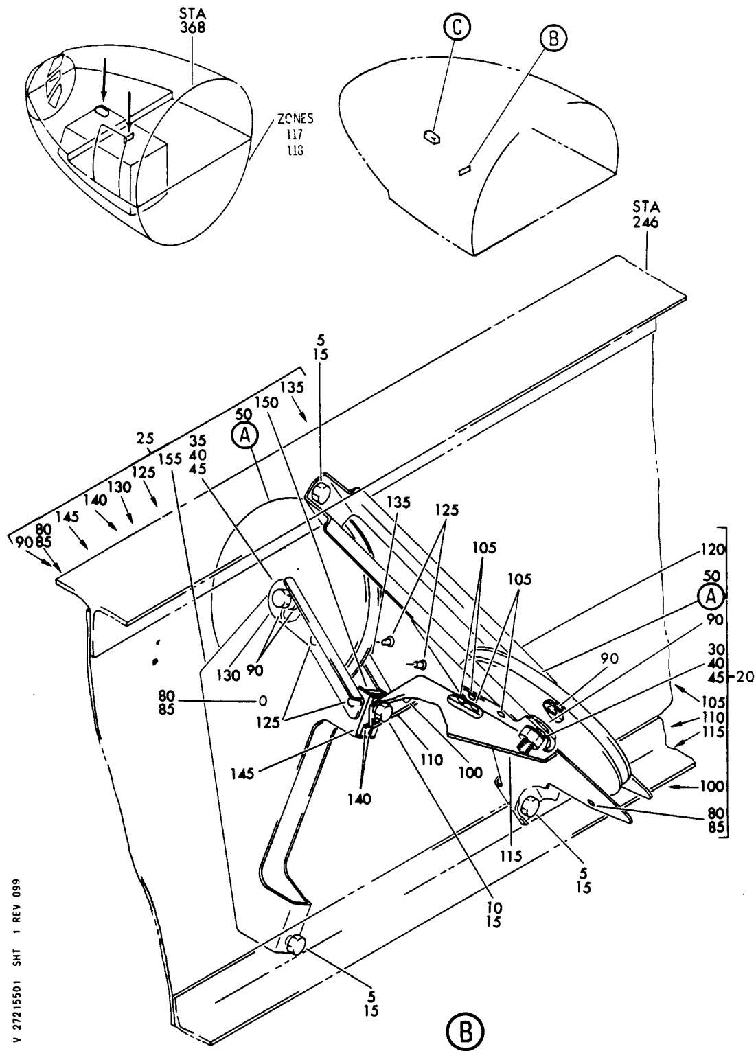
BRACKET INSTL-STA 246.0 RA AND RB CABLE PULLEY FIGURE 1 (SHEET 1)
