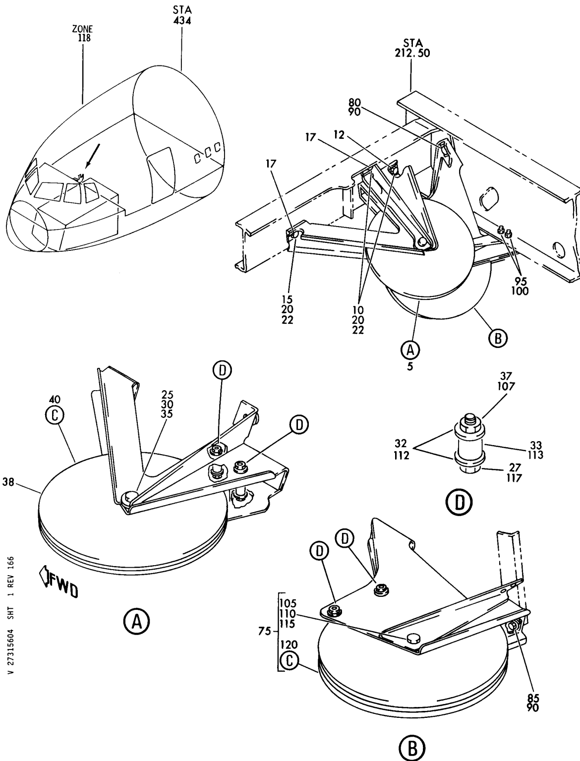
BRACKET INSTL-ELEV E2A AND E2B STA 202-212 PULLEY FIGURE 4 (SHEET 1)
