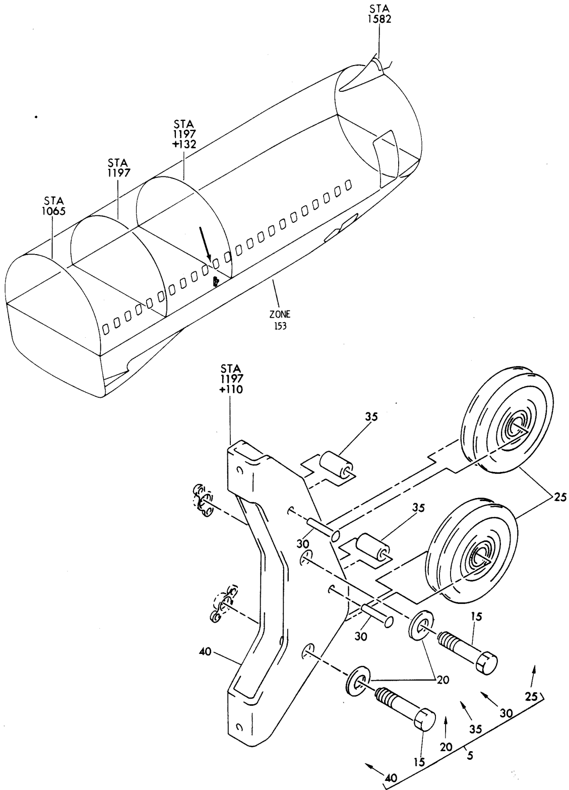
BRACKET INSTL-STA 1197+110 IDLER PULLEY FIGURE 5
