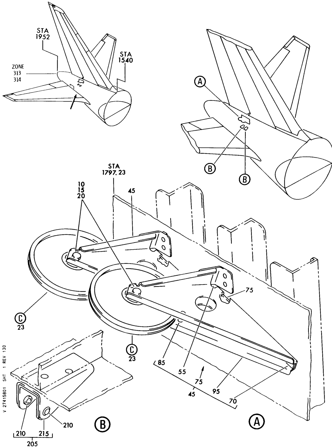
BRACKET INSTL-HORIZ STAB. CONT SYS PULLEY FIGURE 1 (SHEET 1)
