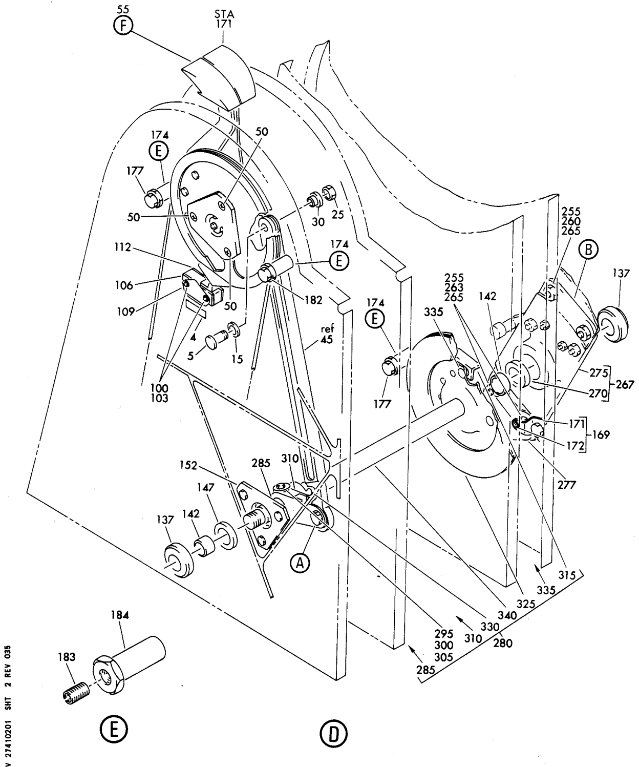
LEVER INSTL-CONT STAND STAB. TRIM FIGURE 1 (SHEET 2)
