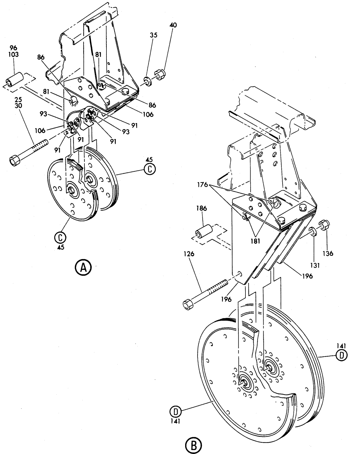
BRACKET INSTL-SECT. 41 PULLEY FIGURE 1 (SHEET 2)
