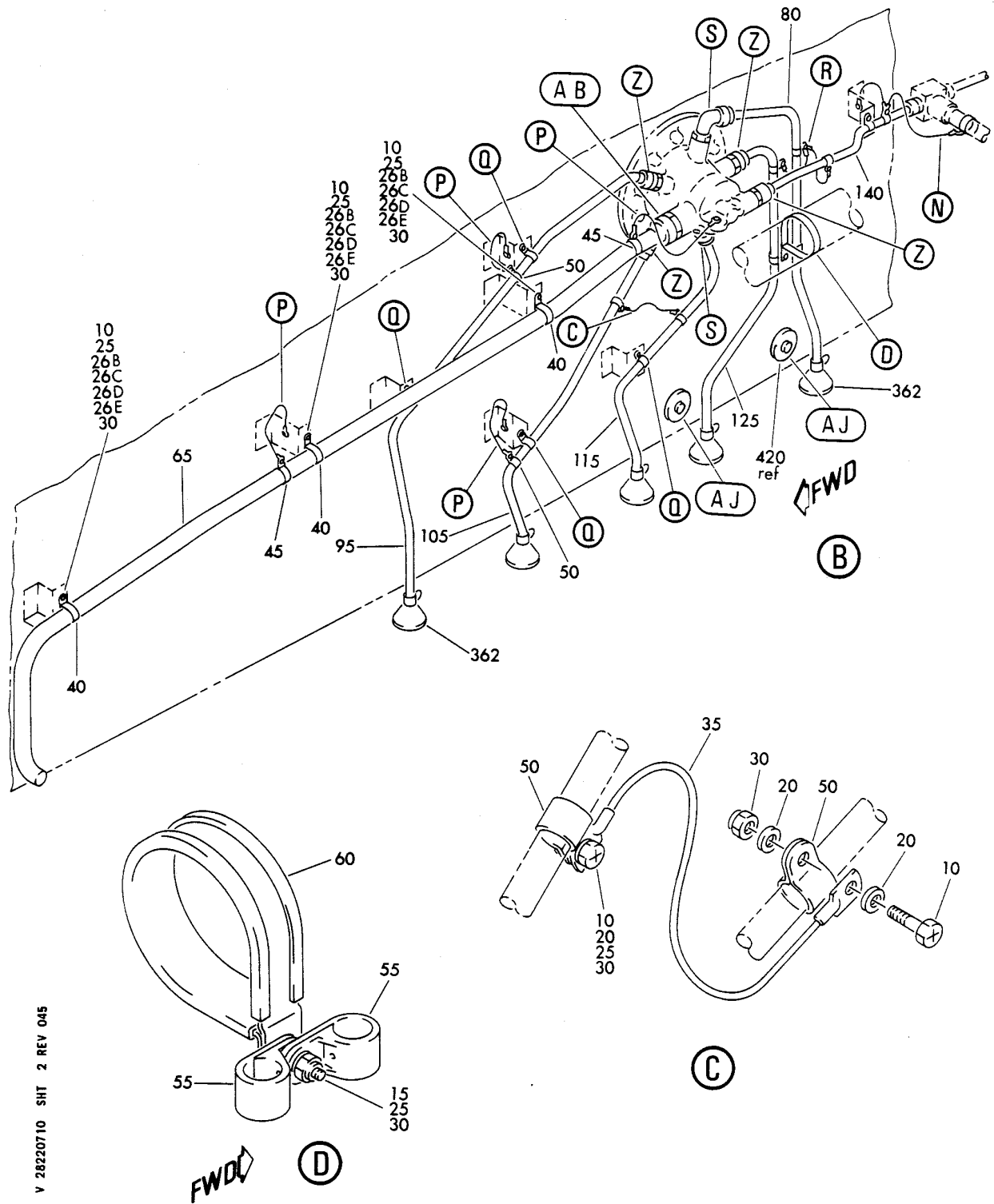
TUBING INSTL-AUTO. SUMPING SYS FIGURE 10 (SHEET 2)
