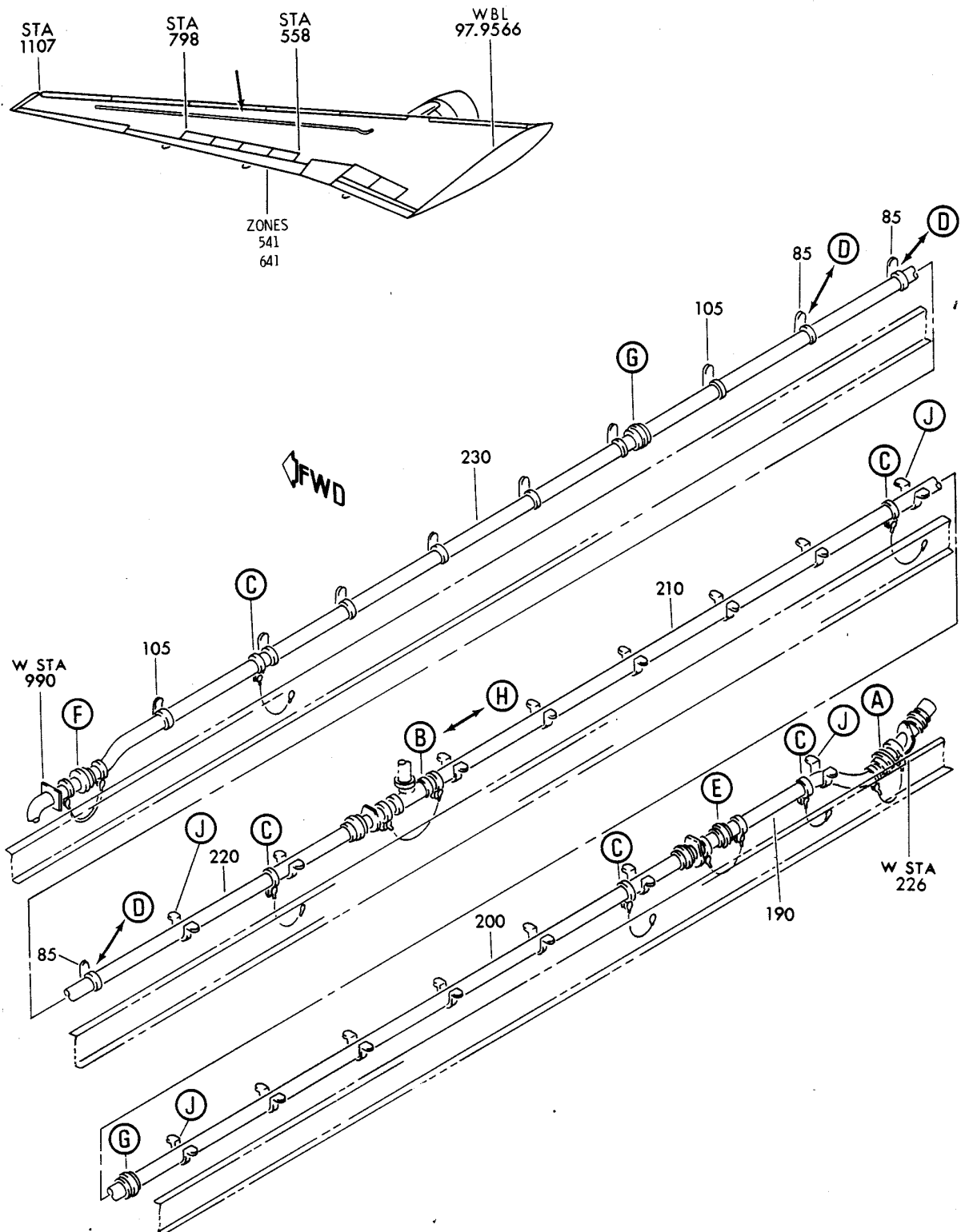
TUBING INSTL-SURGE TANK DRAIN FIGURE 15 (SHEET 1)
