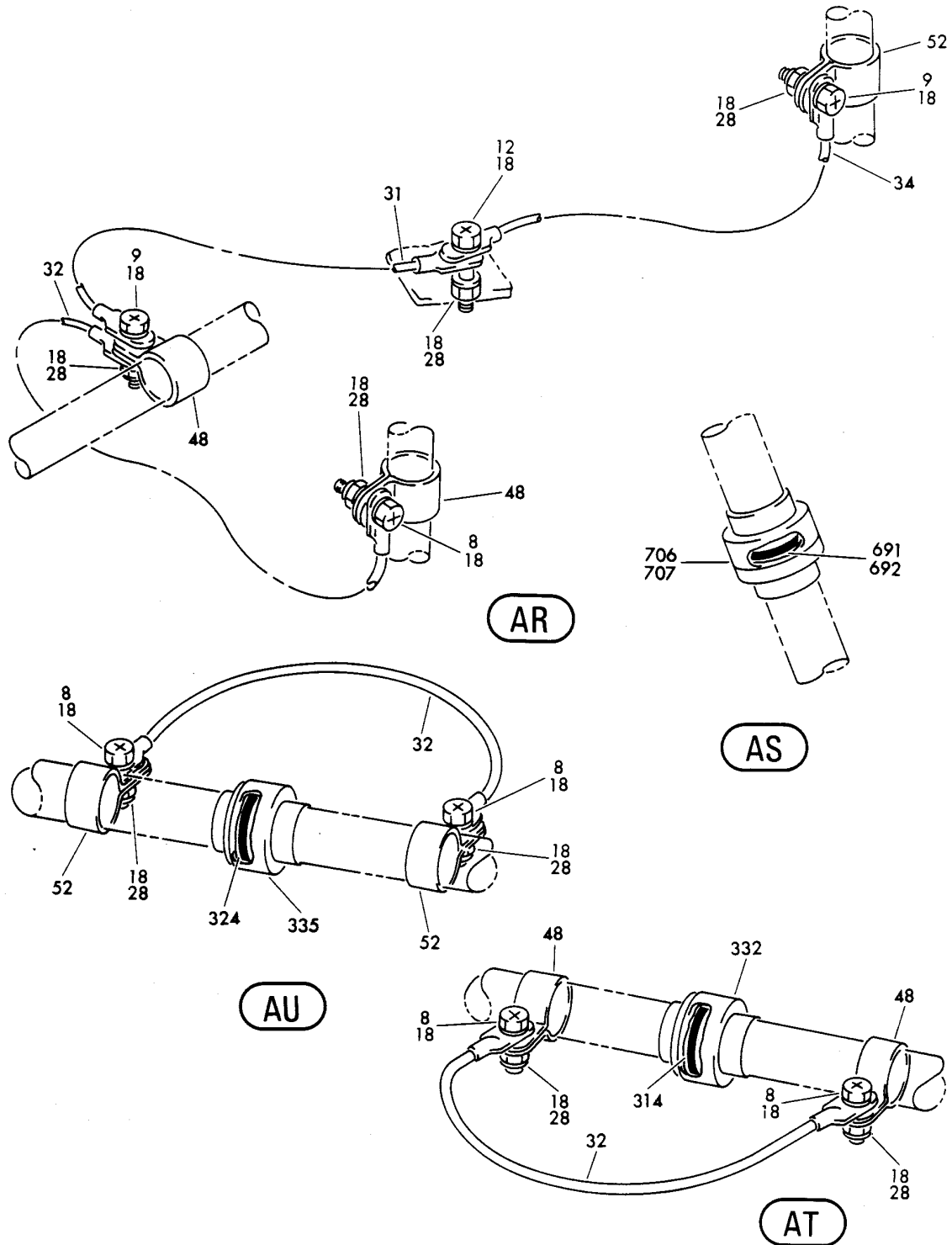
TUBING INSTL-AUTO. SUMPING SYS FIGURE 10 (SHEET 13)
