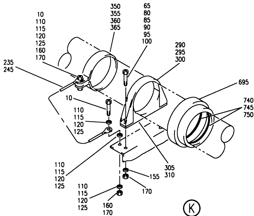
TUBING INSTL-FUELING SYS RIGHT MAIN TANK FIGURE 6 (SHEET 7)
