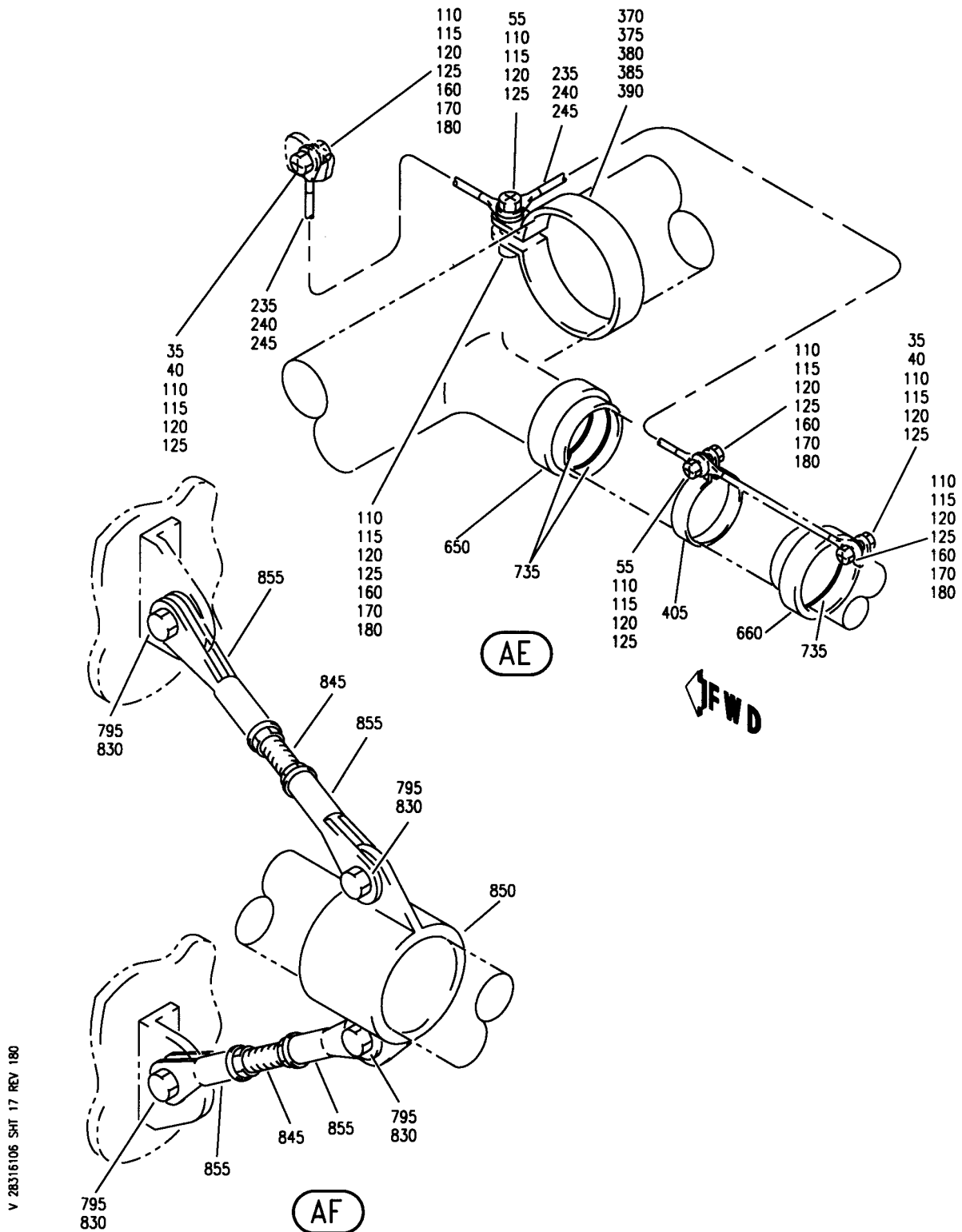
TUBING INSTL-FUELING SYS RIGHT MAIN TANK FIGURE 6 (SHEET 17)
