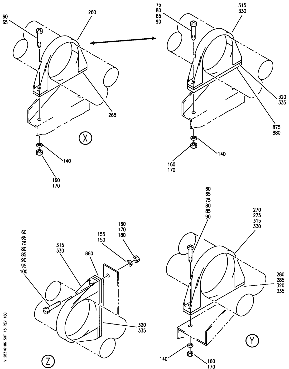
TUBING INSTL-FUELING SYS RIGHT MAIN TANK FIGURE 6 (SHEET 15)
