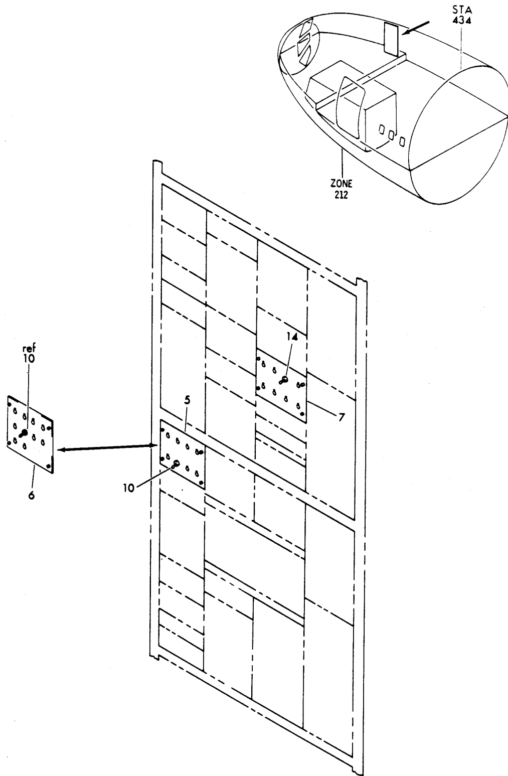
PANEL INSTL-R SIDE (FUEL ONLY) FIGURE 1
