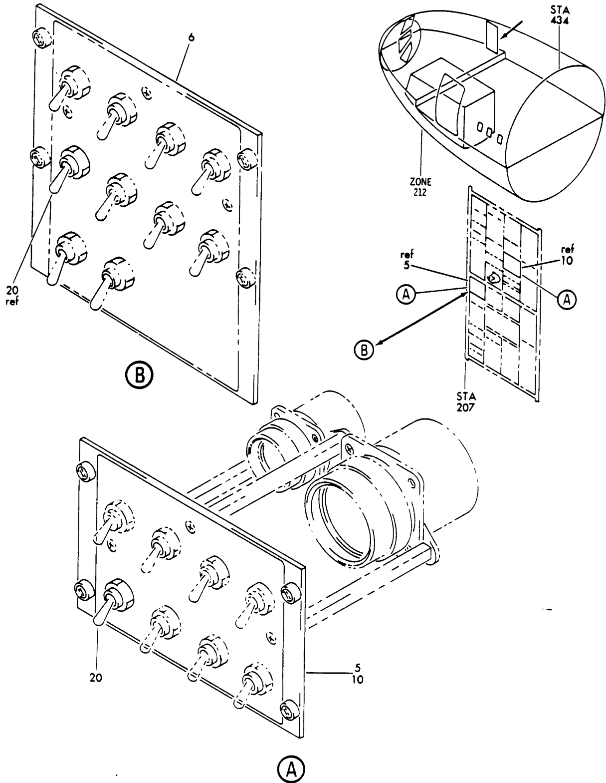
PANEL INSTL-R SIDE (WING THERMAL ANTI-ICING ONLY) FIGURE 1
