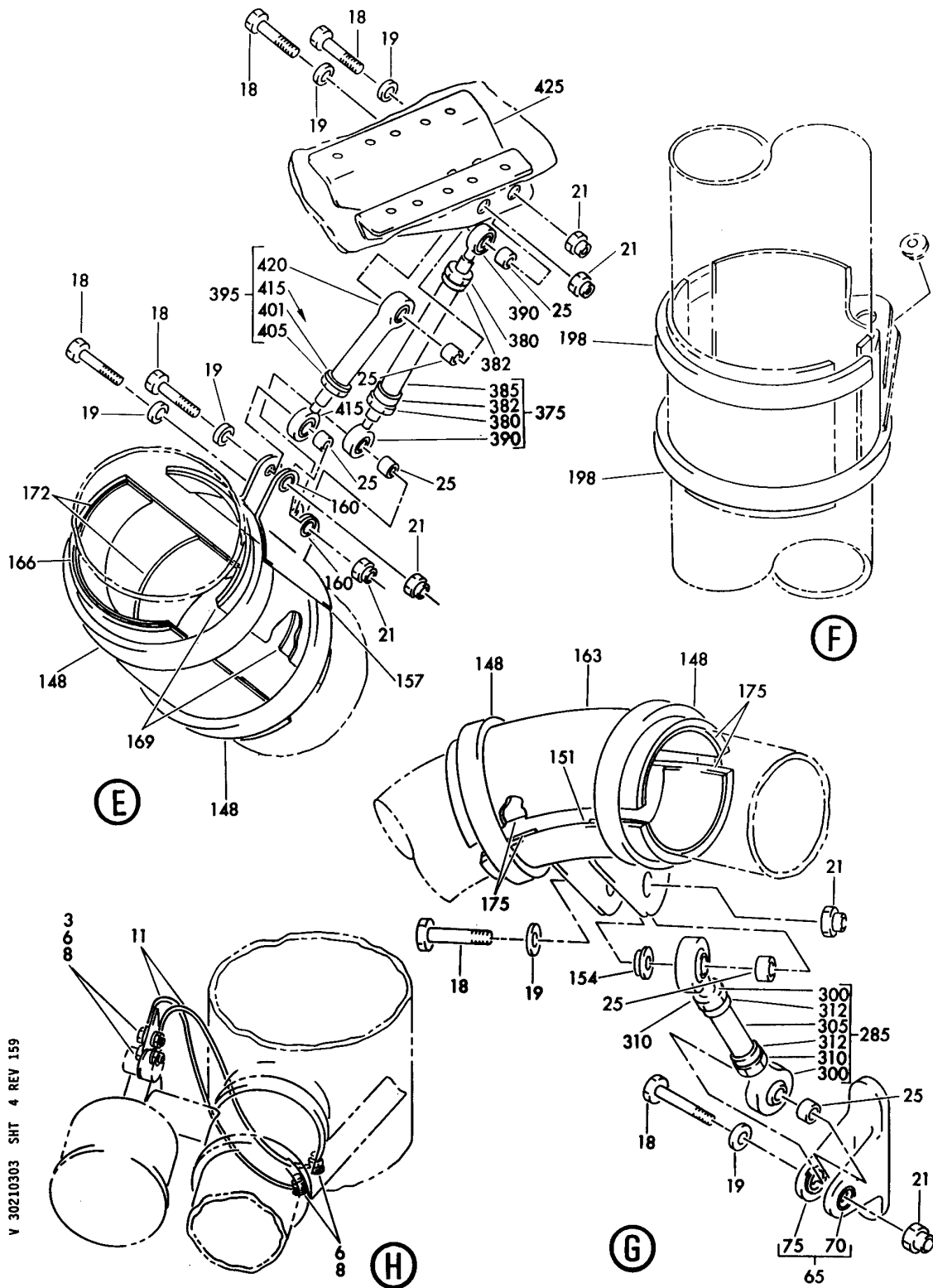
DUCT AND WIRING INSTL-THRM ANTI-ICING INLET FIGURE 3 (SHEET 4)
