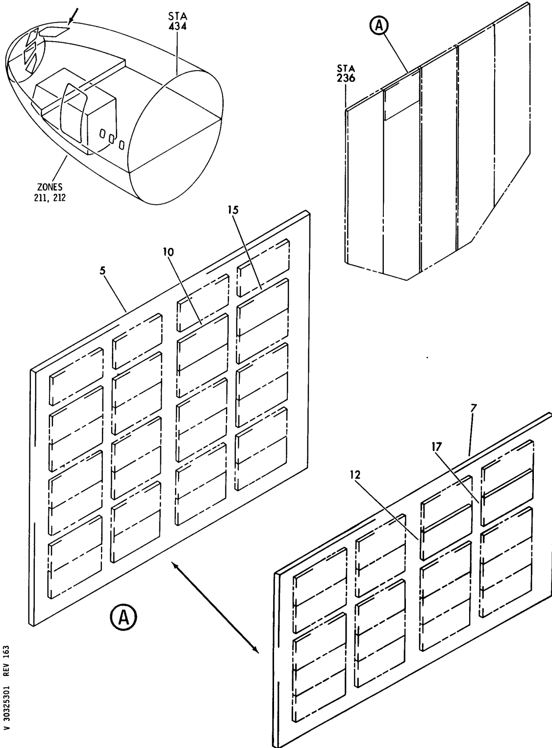
PANEL INSTL-OVHD (ANGLE OF ATTACK PROBE HEAT ONLY) FIGURE 1
