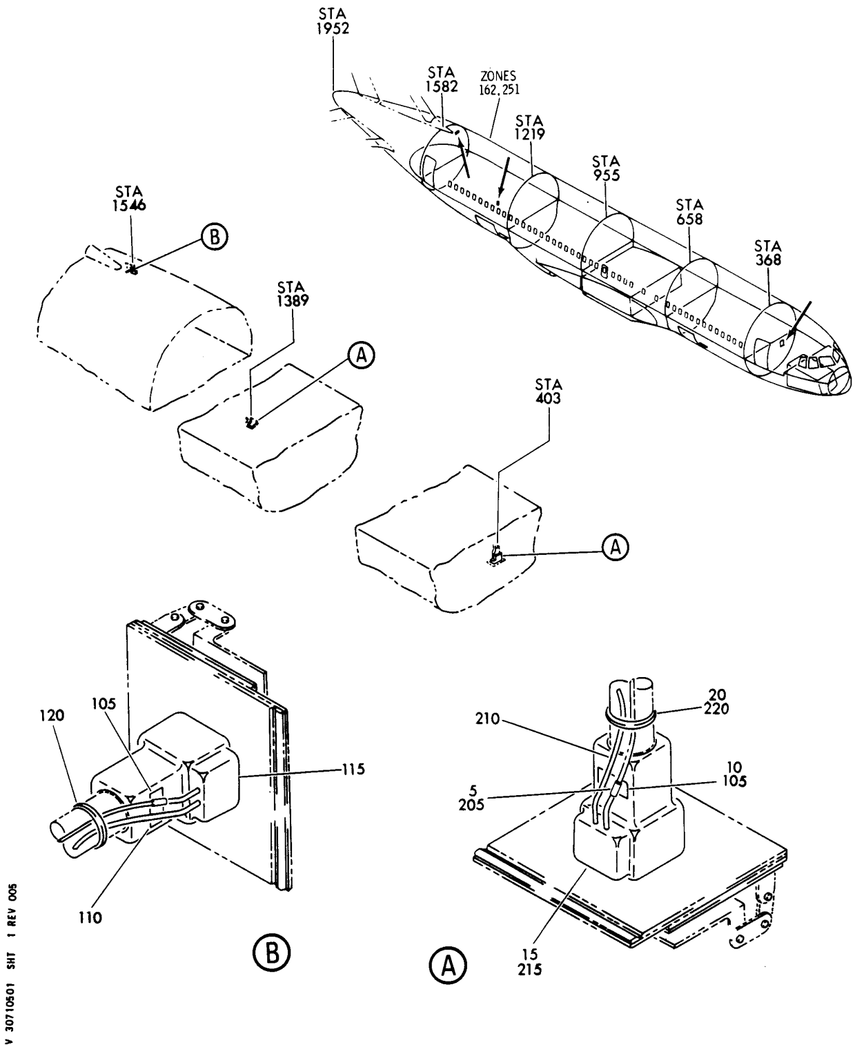
HEATER INSTL-POTABLE WATER SYS FILL FTG FIGURE 1
