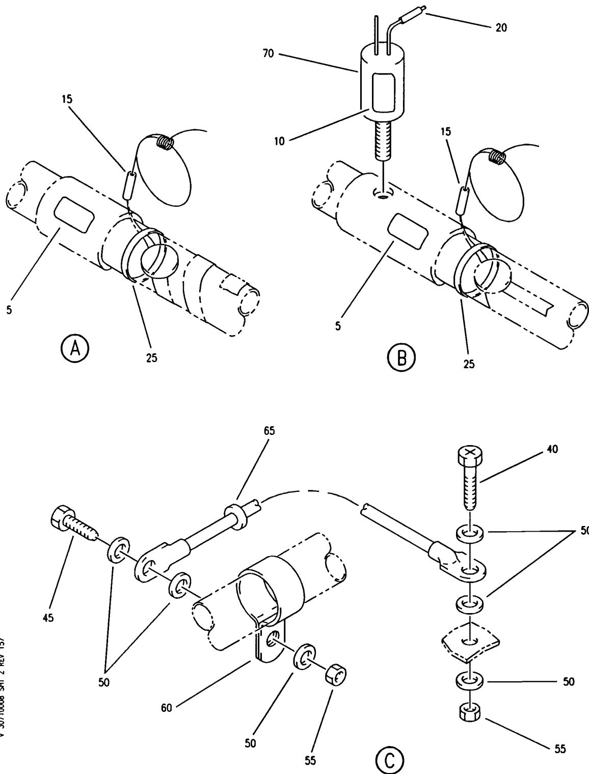
HEATER INSTL-SECT. 46 POTABLE WATER SYS (ICE AND RAIN PROTECTION ONLY) FIGURE 8 (SHEET 2)
