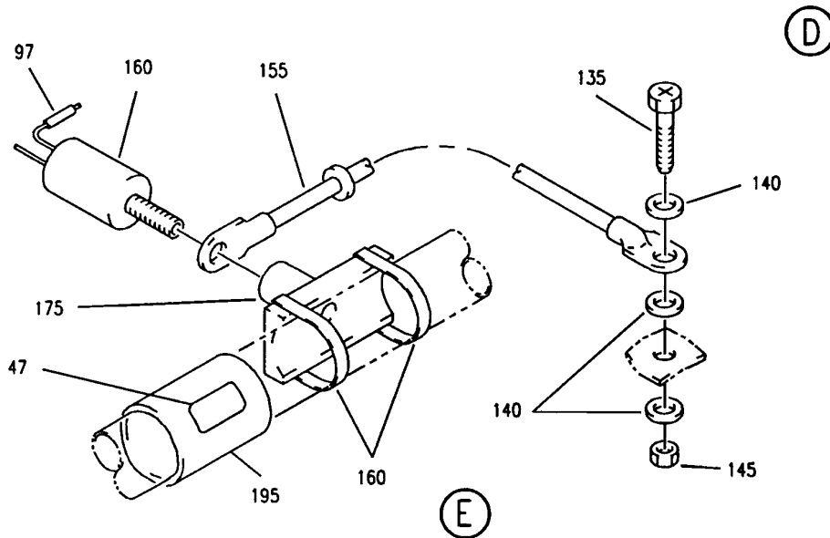
HEATER INSTL-SECT. 46 POTABLE WATER SYS (ICE AND RAIN PROTECTION ONLY) FIGURE 12 (SHEET 3)
