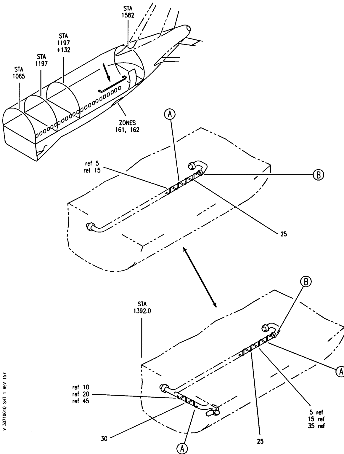
HEATER INSTL-SECT. 46 POTABLE WATER SYS (ICE AND RAIN PROTECTION ONLY) FIGURE 10 (SHEET 1)
