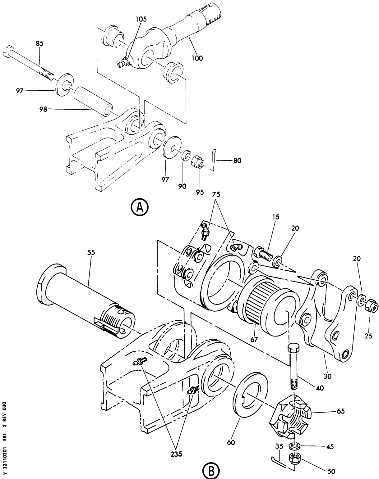
STRUT ASSY-SIDE FIGURE 1 (SHEET 2)
