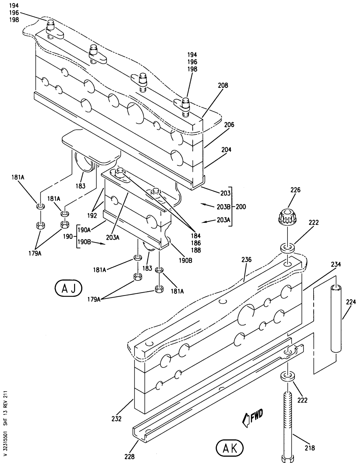
HYDRAULIC INSTL-SECT. 45 (LANDING GEAR CONTROL ONLY) FIGURE 1 (SHEET 13)
