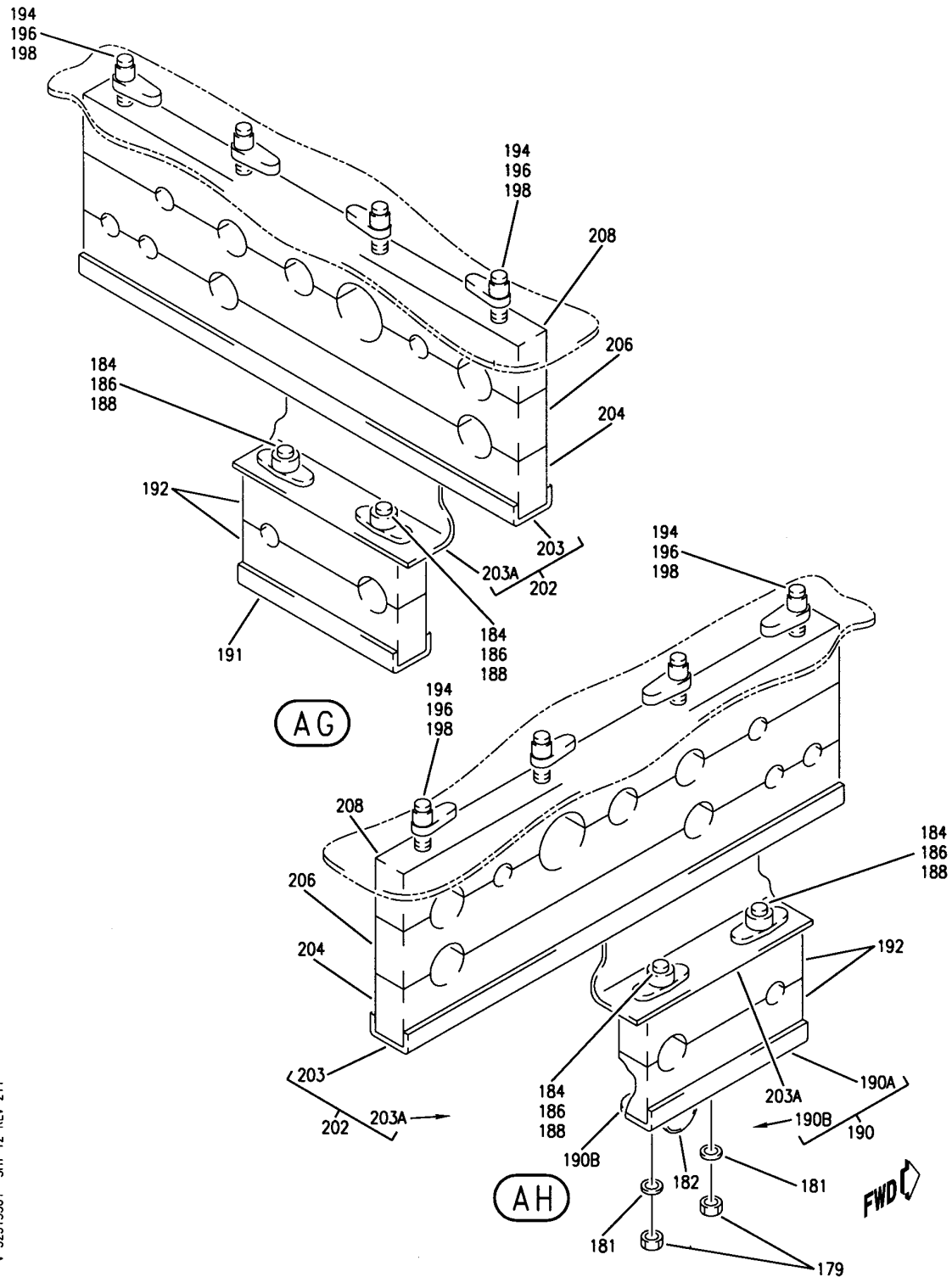
HYDRAULIC INSTL-SECT. 45 (LANDING GEAR CONTROL ONLY) FIGURE 1 (SHEET 12)
