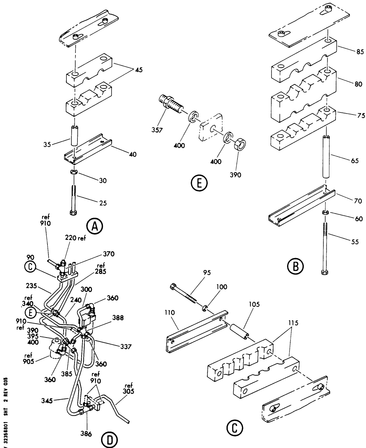
HYDRAULIC INSTL-SECT. 45 (LANDING GEAR ALTERNATE EXTEND SYSTEM ONLY) FIGURE 1 (SHEET 2)
