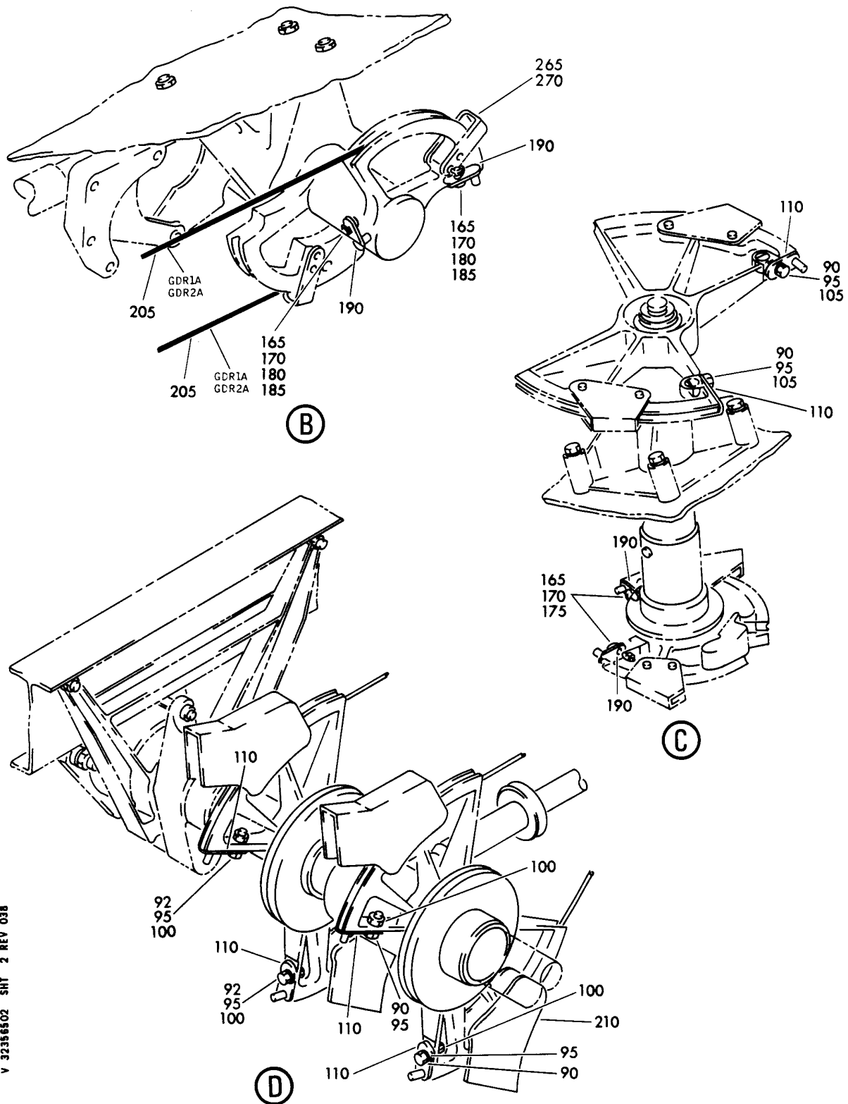
CONTROL INSTL-ALTERNATE EXTEND LG FIGURE 2 (SHEET 2)
