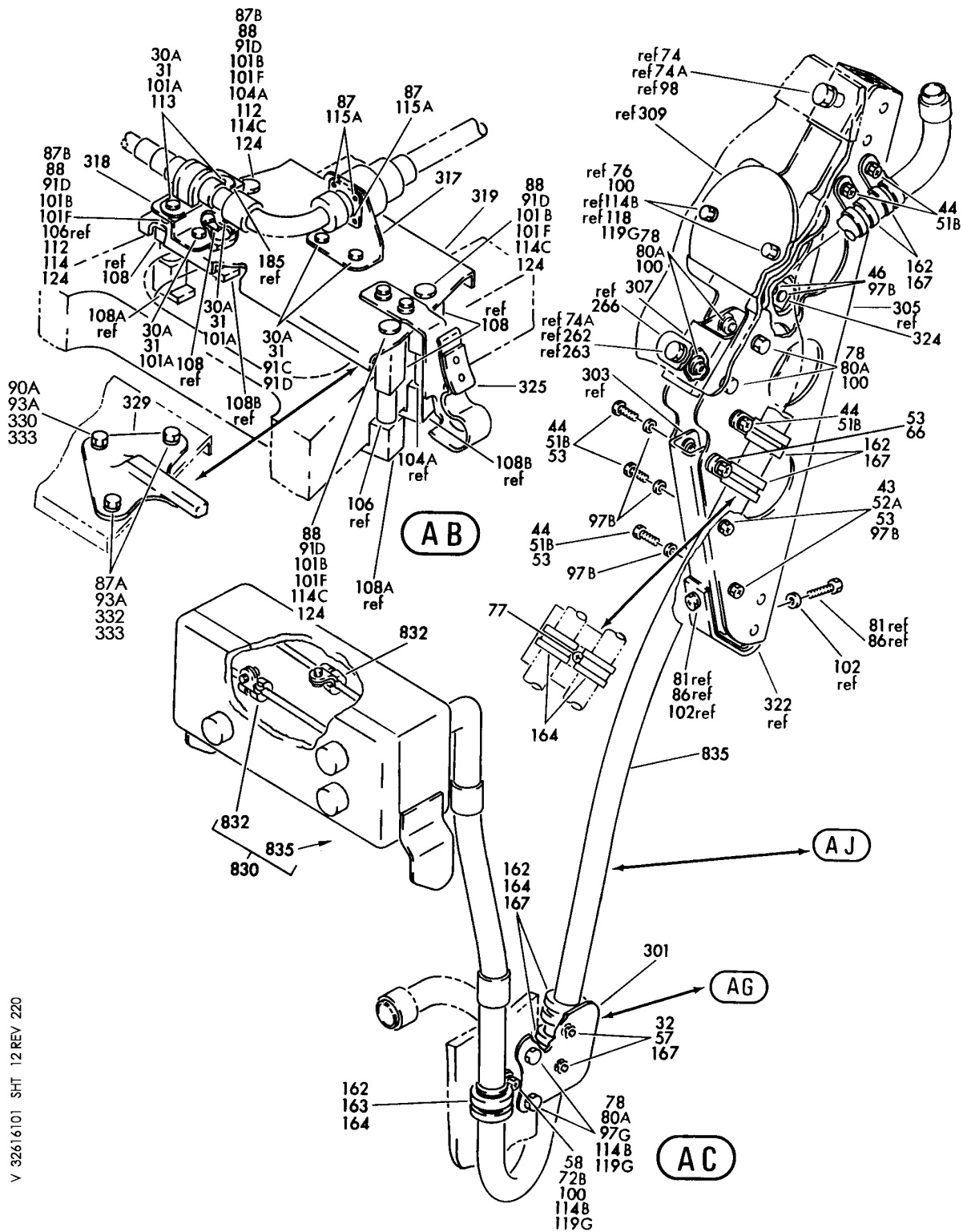
GEAR ASSY-NOSE LDG (POSITION AND WARNING ONLY) FIGURE 1 (SHEET 12)
