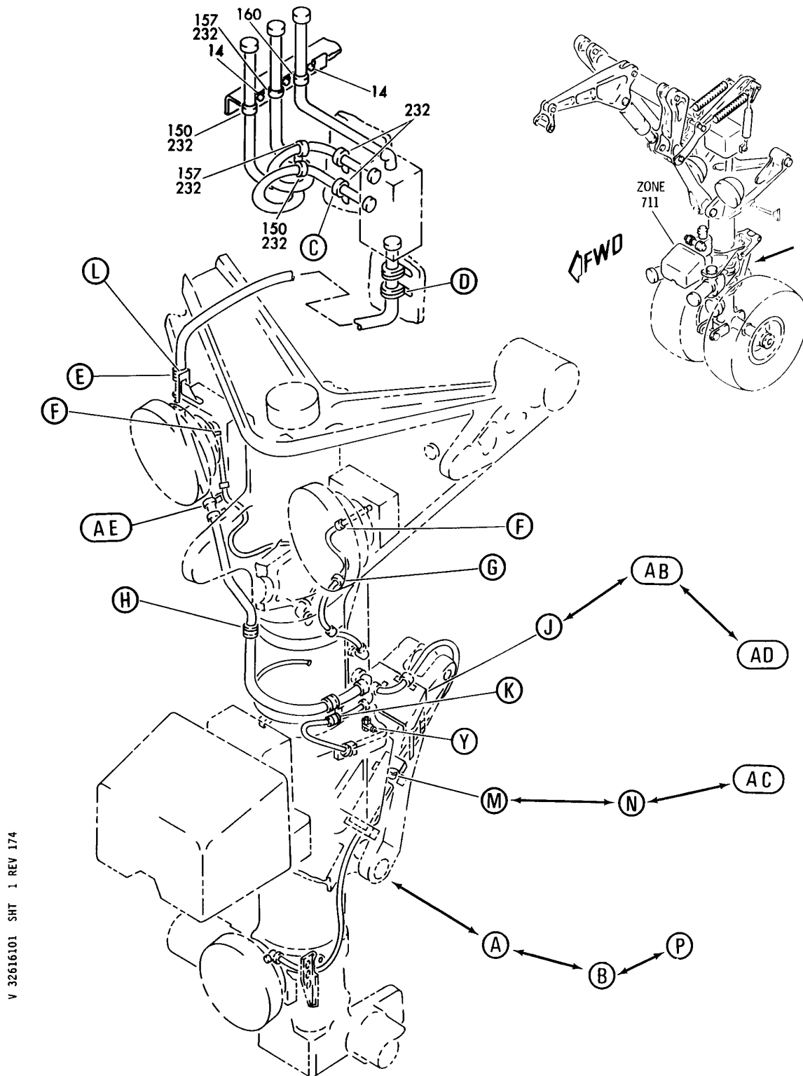
GEAR ASSY-NOSE LDG (POSITION AND WARNING ONLY) FIGURE 1 (SHEET 1)
