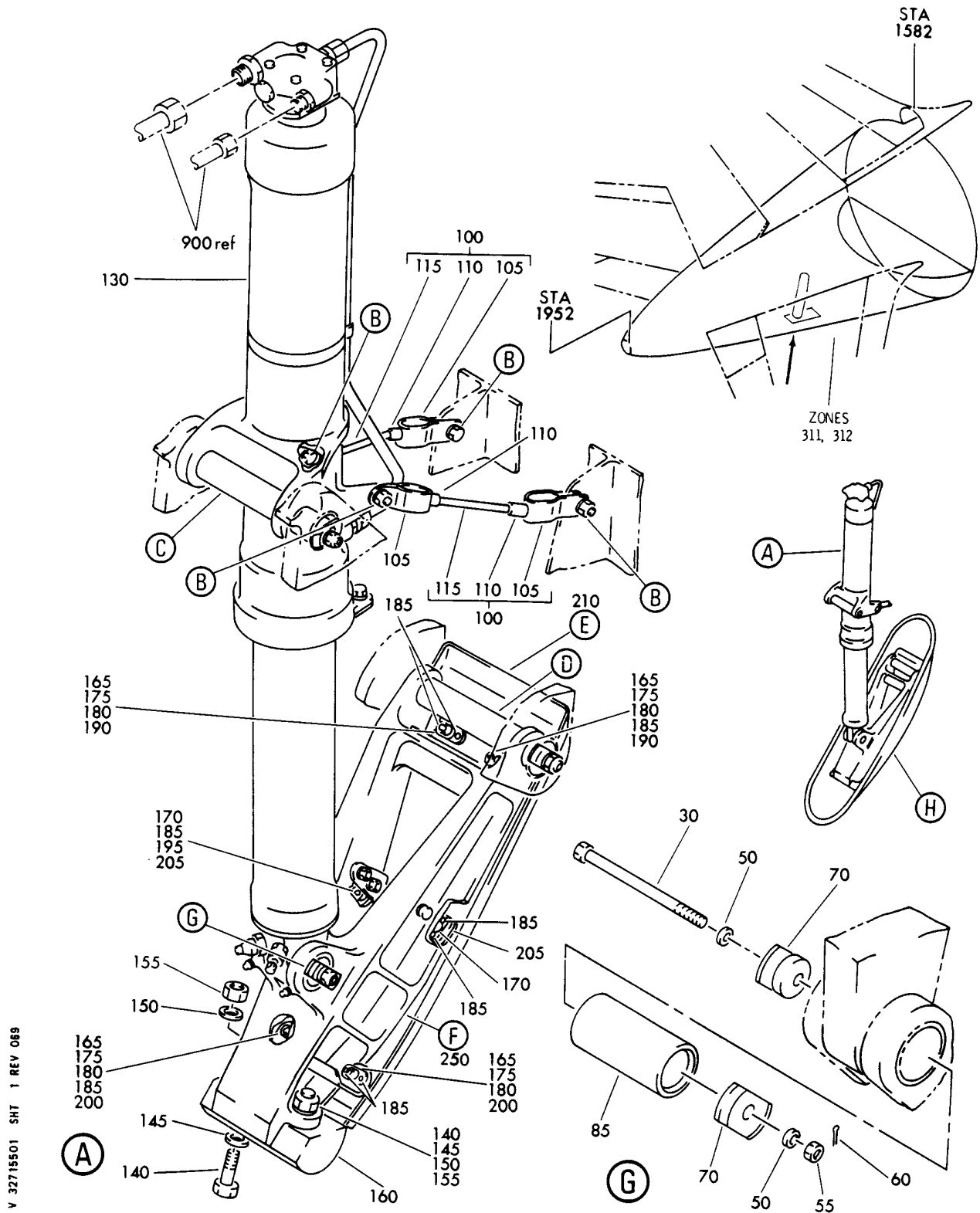
TAIL SKID INSTL AND FAIRING AND SUPPORT INSTL-767-300 FIGURE 1 (SHEET 1)
