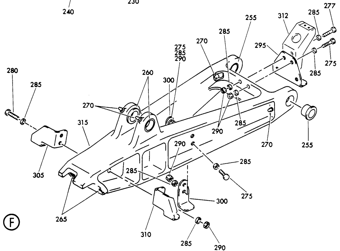
TAIL SKID INSTL AND FAIRING AND SUPPORT INSTL-767-300 FIGURE 1 (SHEET 3)
