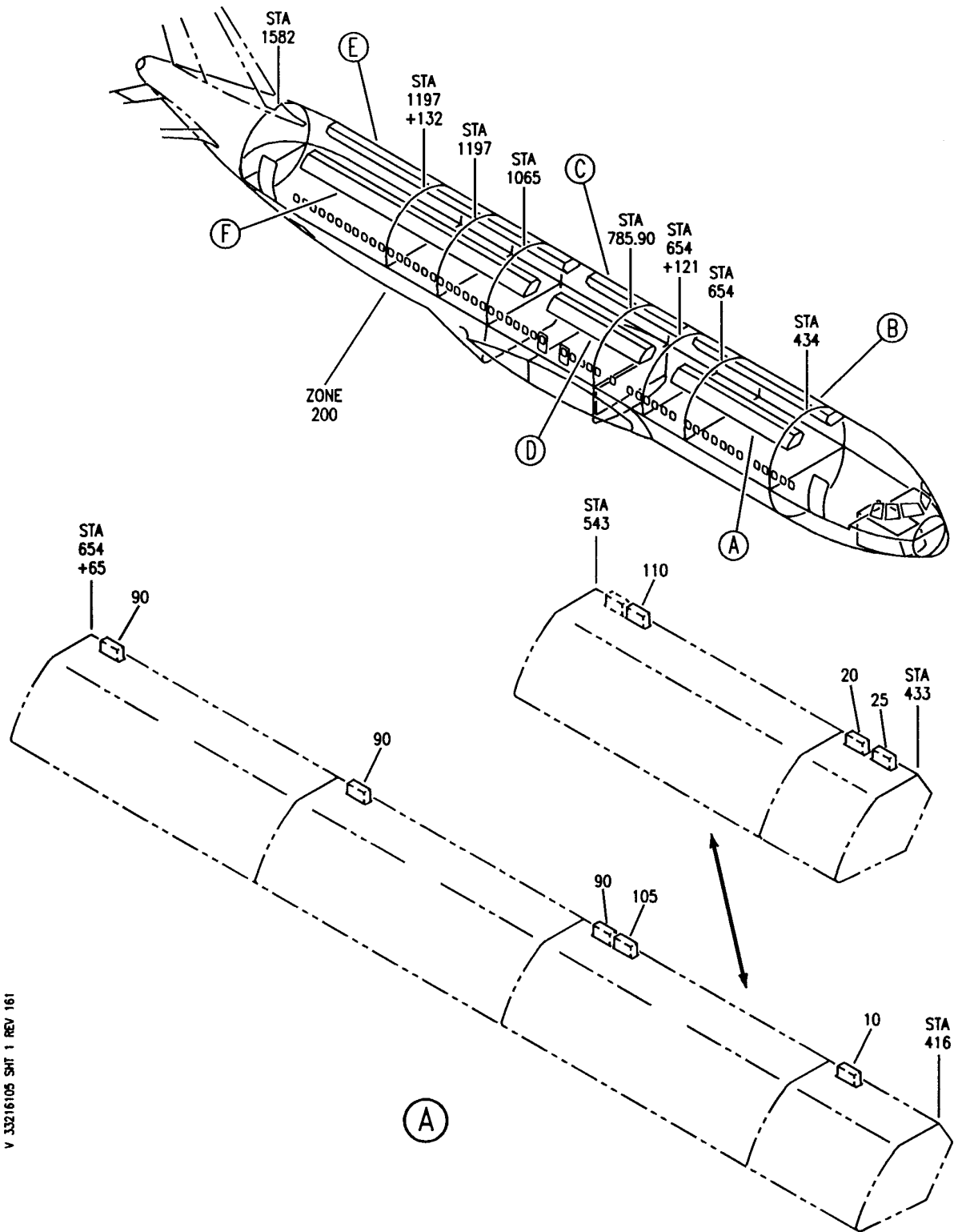
MODULE ASSY-OUTBD OVERHEAD STORAGE BIN (LIGHTS ONLY) FIGURE 5 (SHEET 1)
