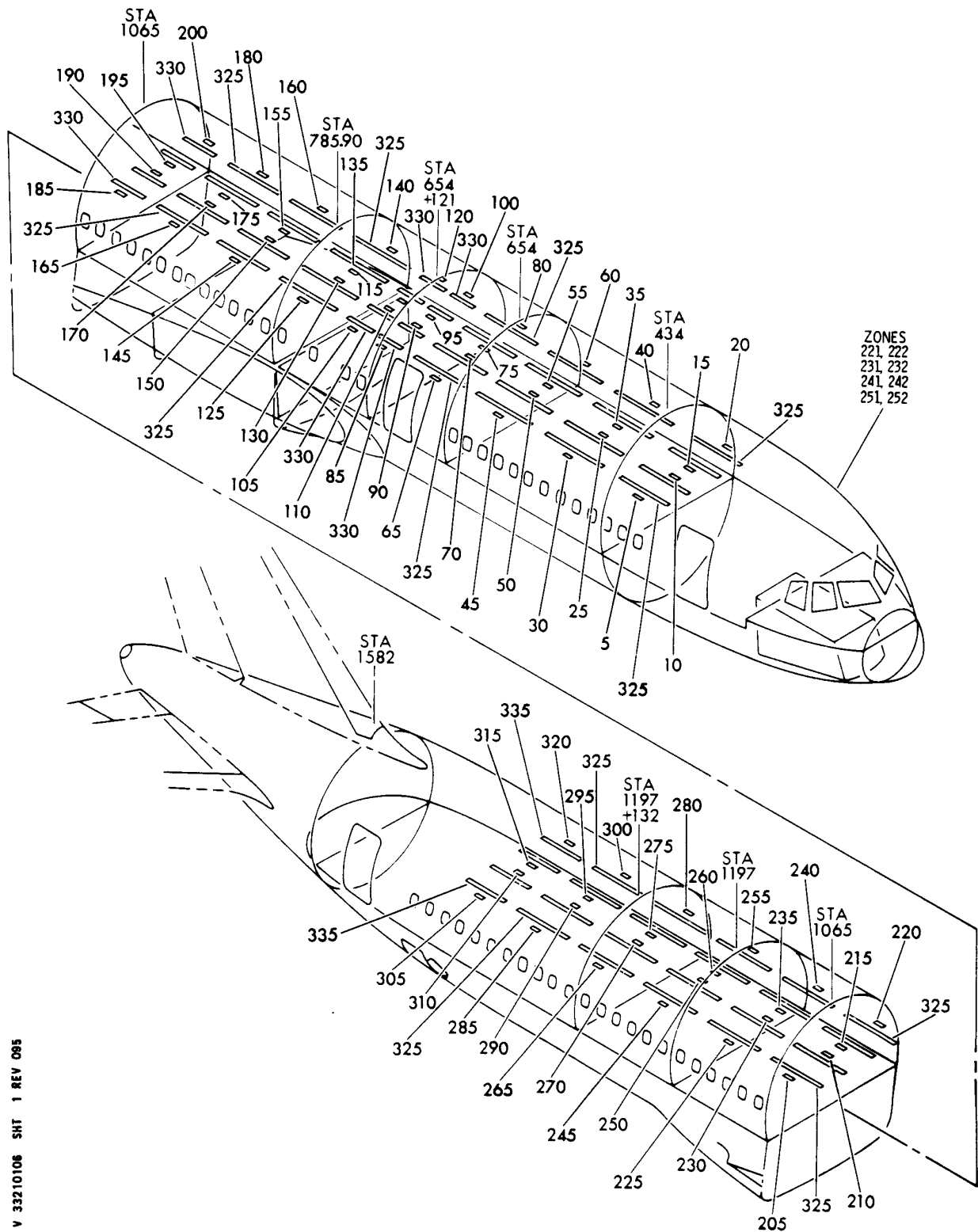
LAMP INSTL-INDIRECT CLG LT FIGURE 6
