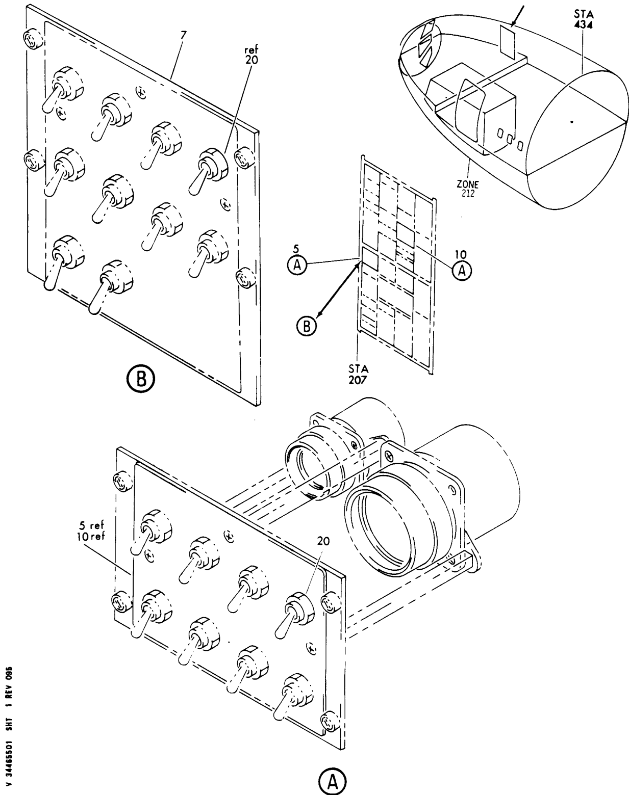
PANEL INSTL-R SIDE (GROUND PROXIMITY WARNING SYSTEM ONLY)
