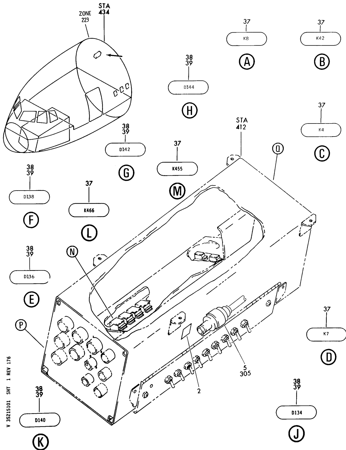
BOX INSTL-FWD LIGHTING PNL (P19) (OXYGEN ONLY) FIGURE 1 (SHEET 1)
