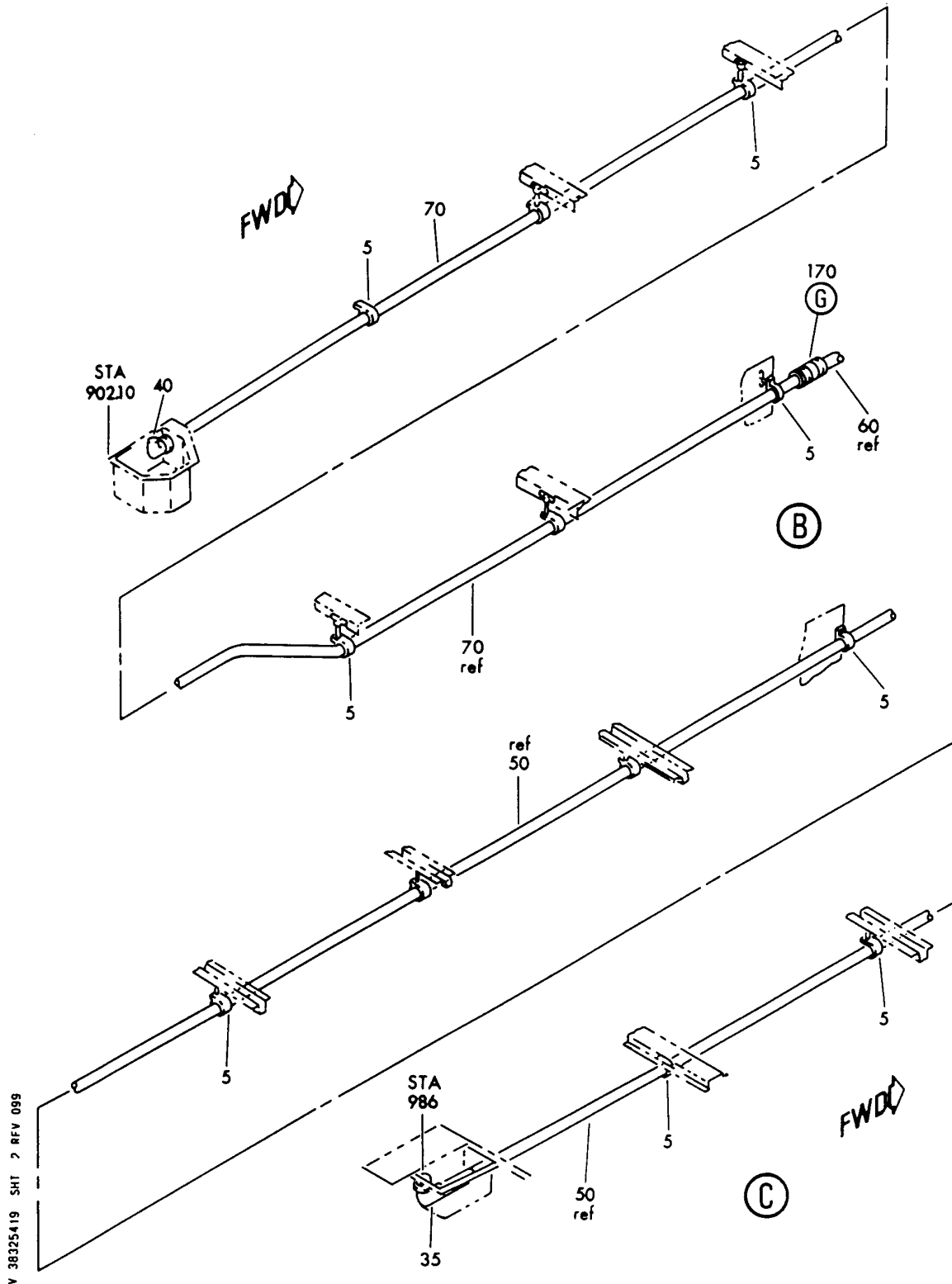
PLUMBING INSTL-SECT. 45 WATER (TOILET SYSTEM ONLY) FIGURE 19 (SHEET 2)
