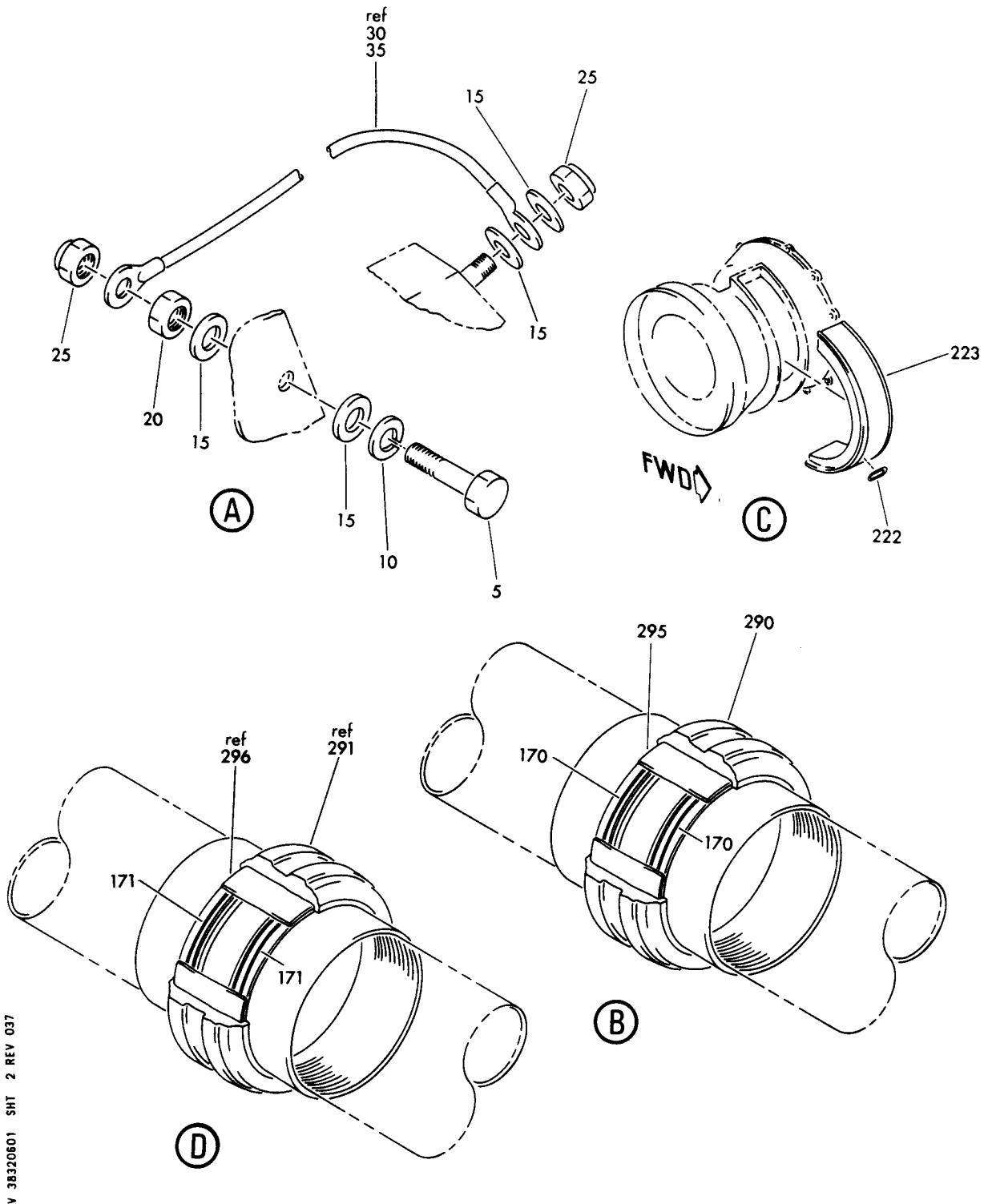
VENT INSTL-WASTE SYS WASTE TANK BLOWER AND OVERBOARD FIGURE 1 (SHEET 2)
