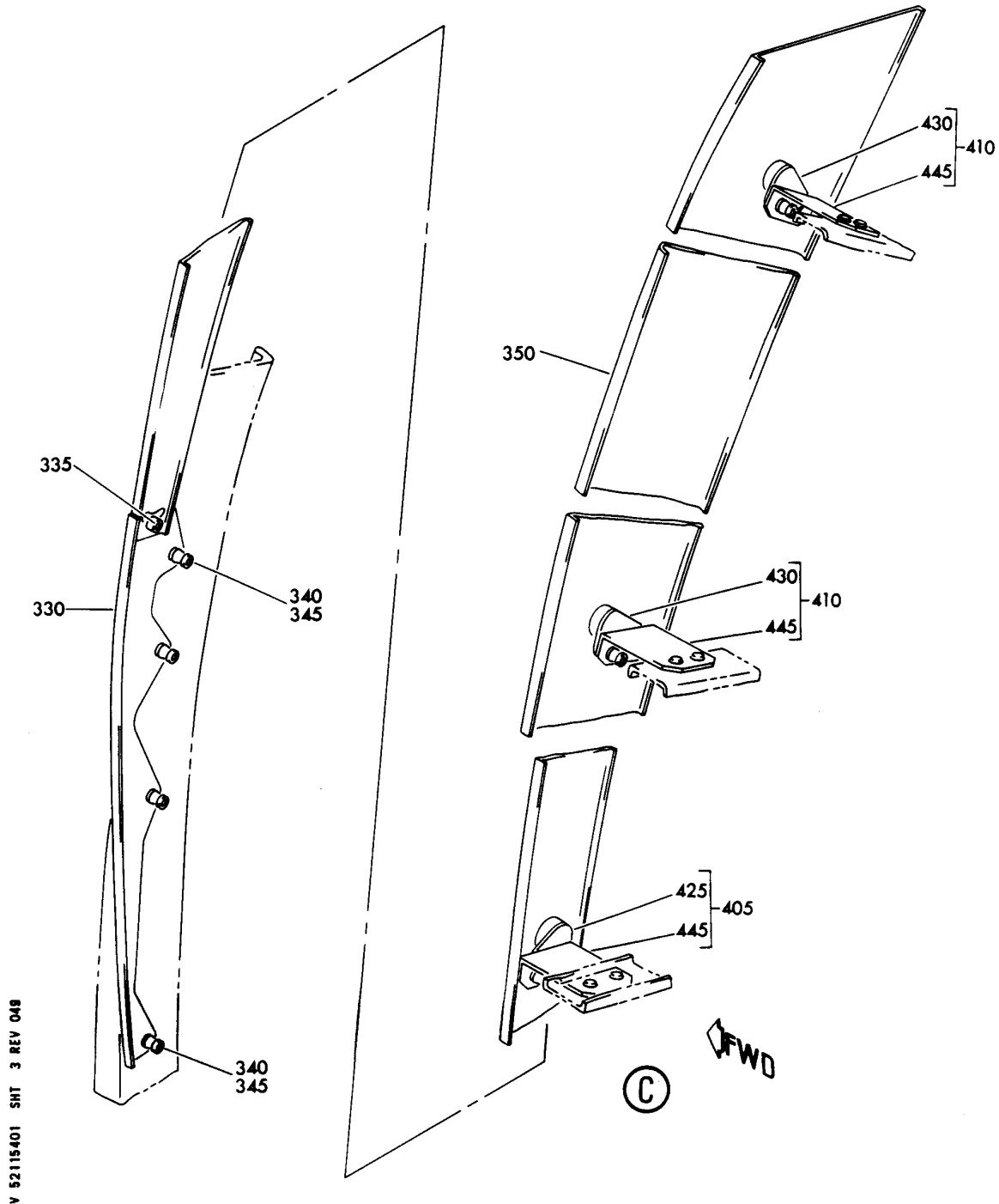
SHROUD INSTL-AFT ENTRY AND SVCE DOOR LWR FIGURE 1 (SHEET 3)
