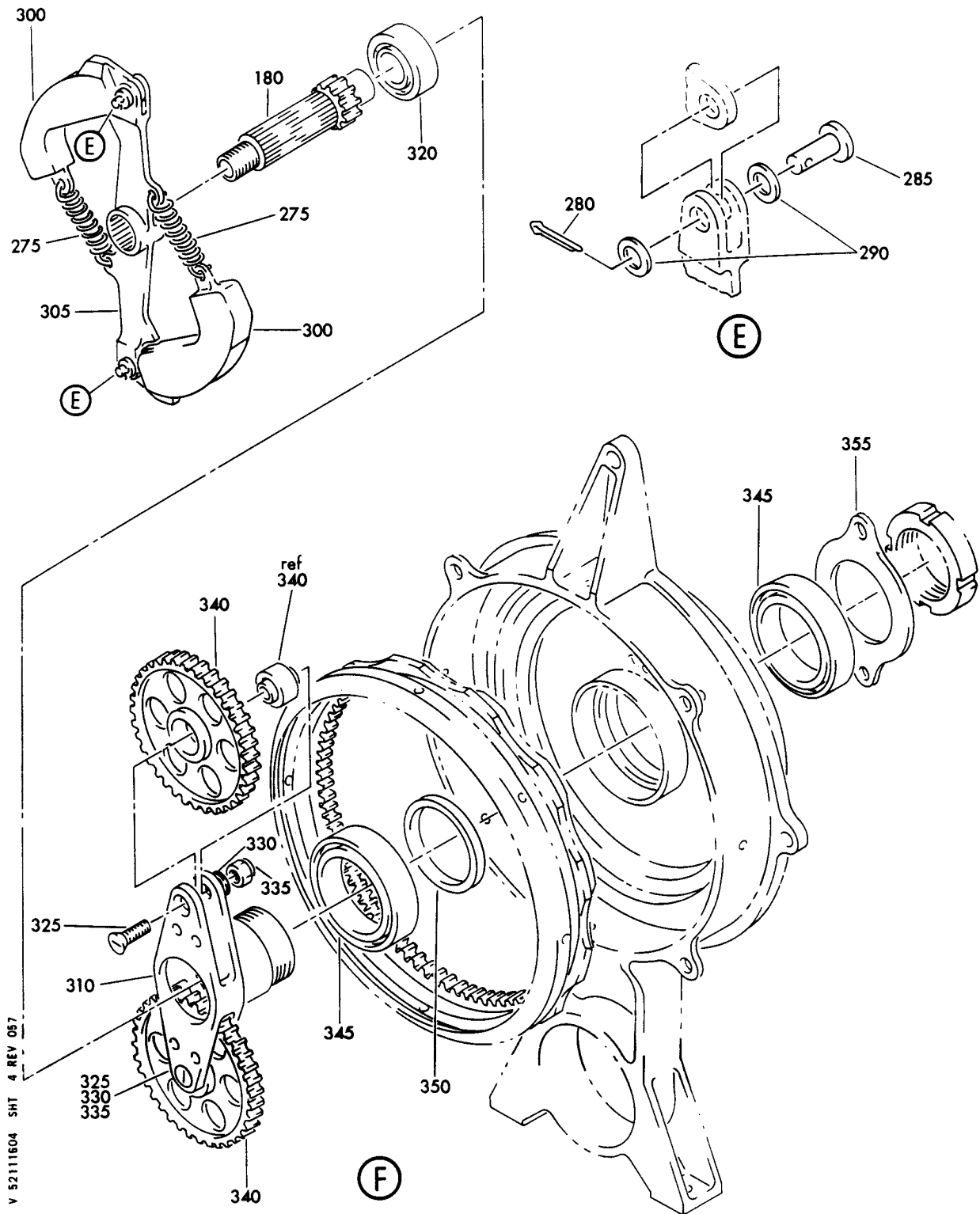
COUNTERBALANCE ASSY-ENTRY AND SERVICE DOOR (DOORS ONLY) FIGURE 4 (SHEET 4)
