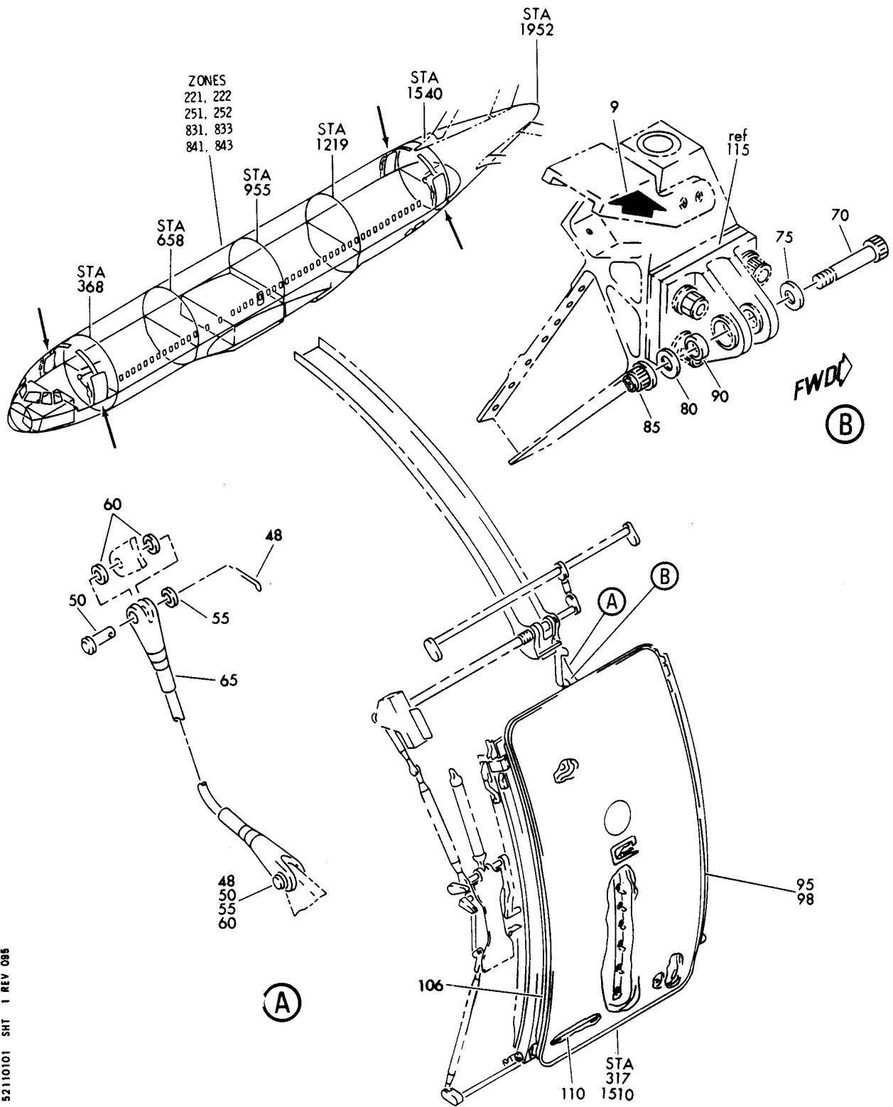
DOOR INTEGRATION-ENTRY AND SVCE FWD AND AFT FIGURE 1
