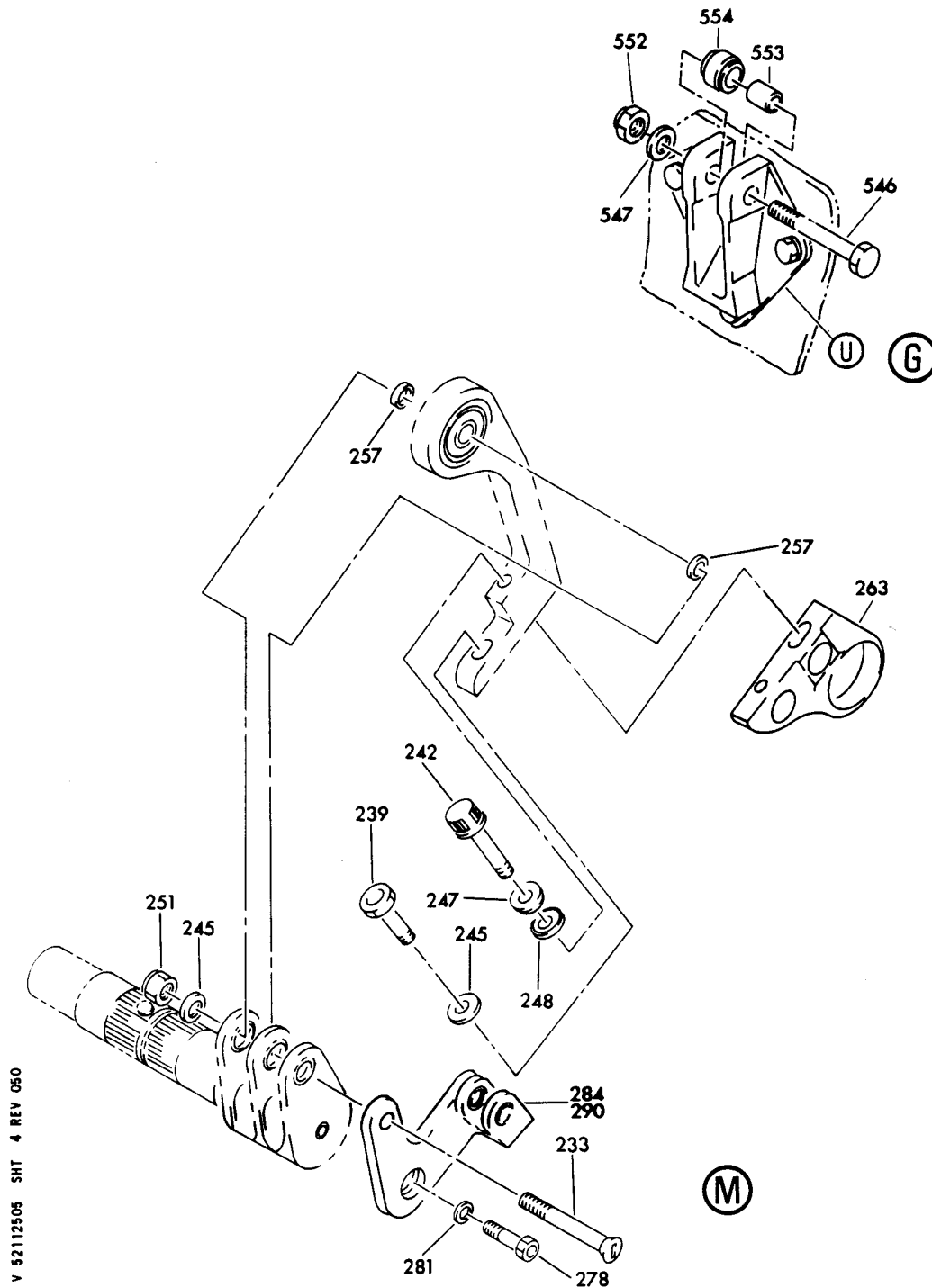
MECHANISM INSTL-ENTRY AND SVCE DOOR HANDLE FIGURE 5 (SHEET 4)
