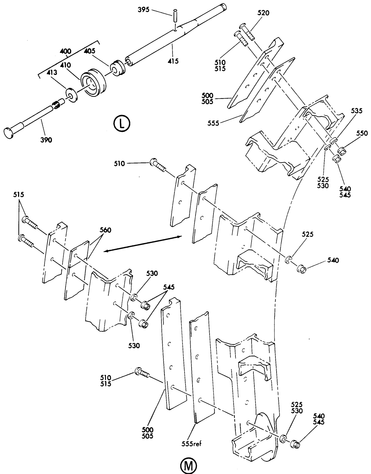
DOOR ASSY-FWD FIGURE 5 (SHEET 5)
