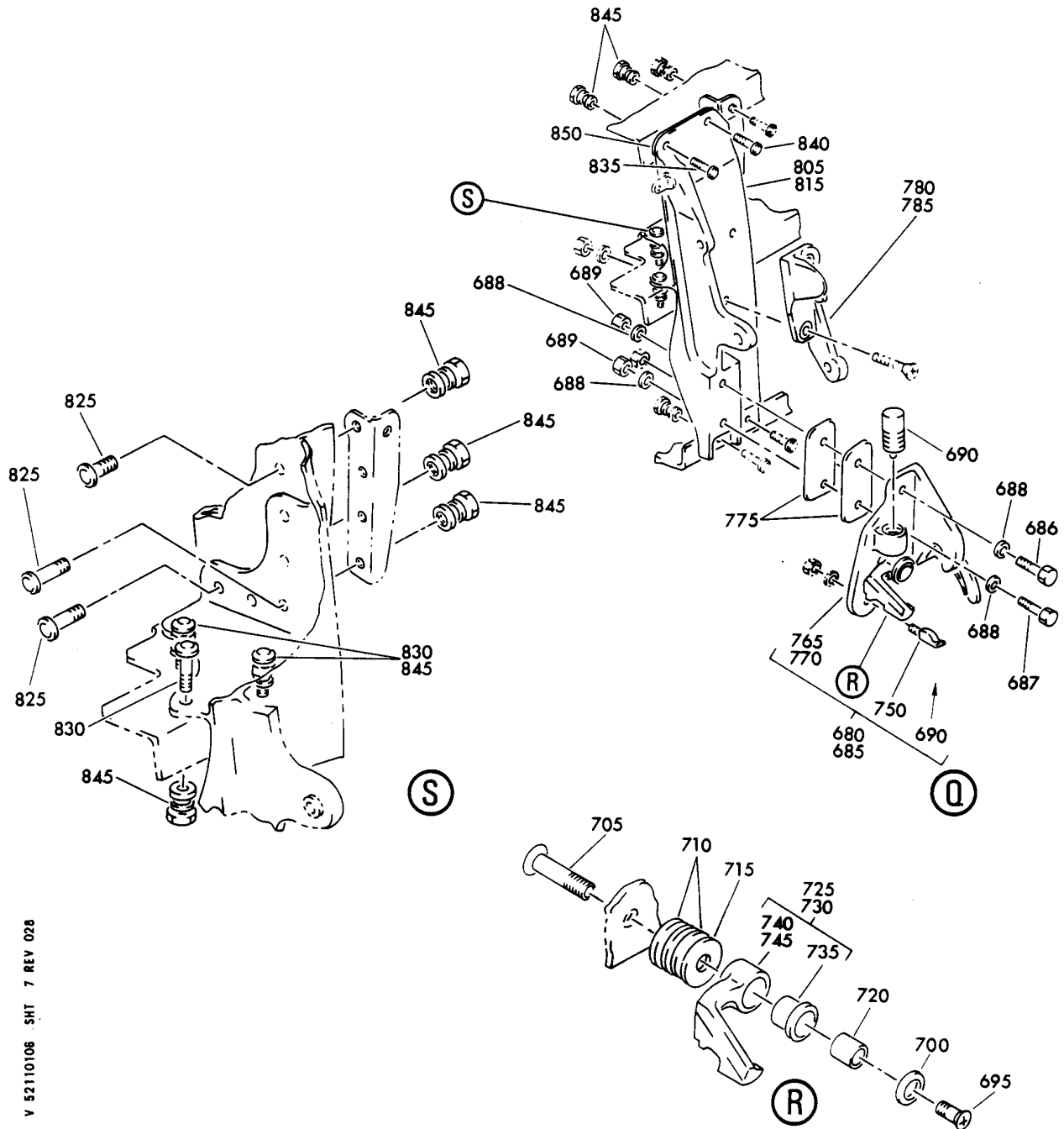
DOOR ASSY-AFT FIGURE 6 (SHEET 7)
