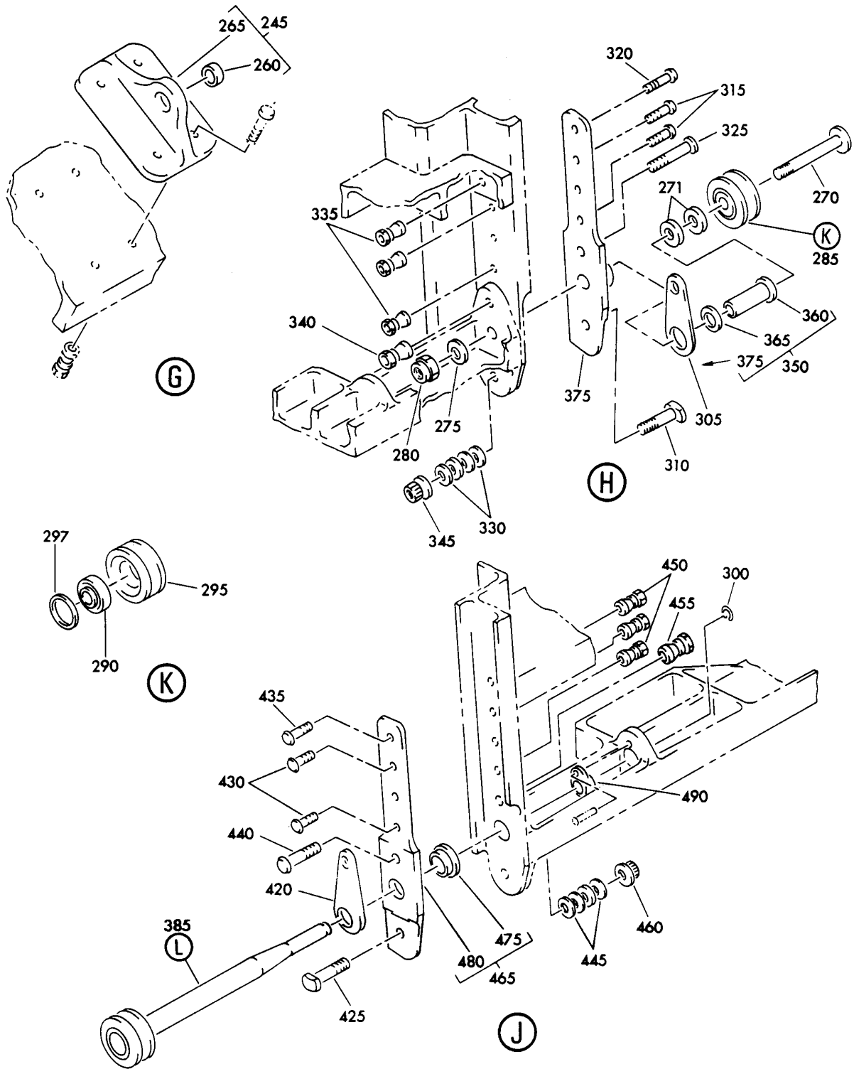
DOOR ASSY-FWD FIGURE 5 (SHEET 4)
