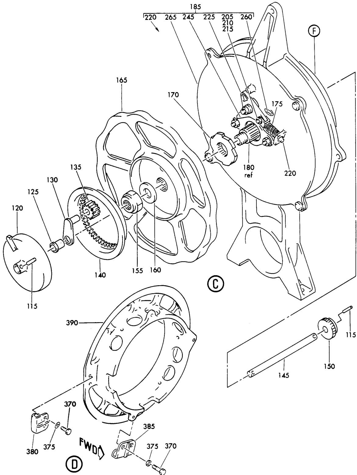
COUNTERBALANCE ASSY-ENTRY AND SERVICE DOOR (DOORS ONLY) FIGURE 4 (SHEET 3)
