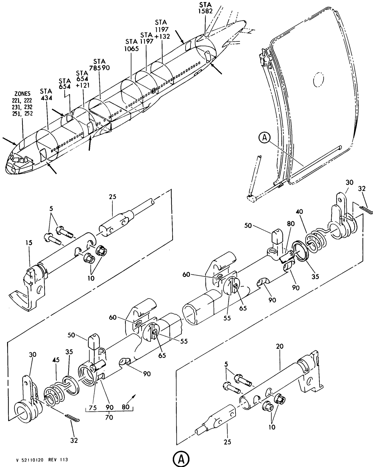
CARRIER ASSY-GIRT BAR FIGURE 20
