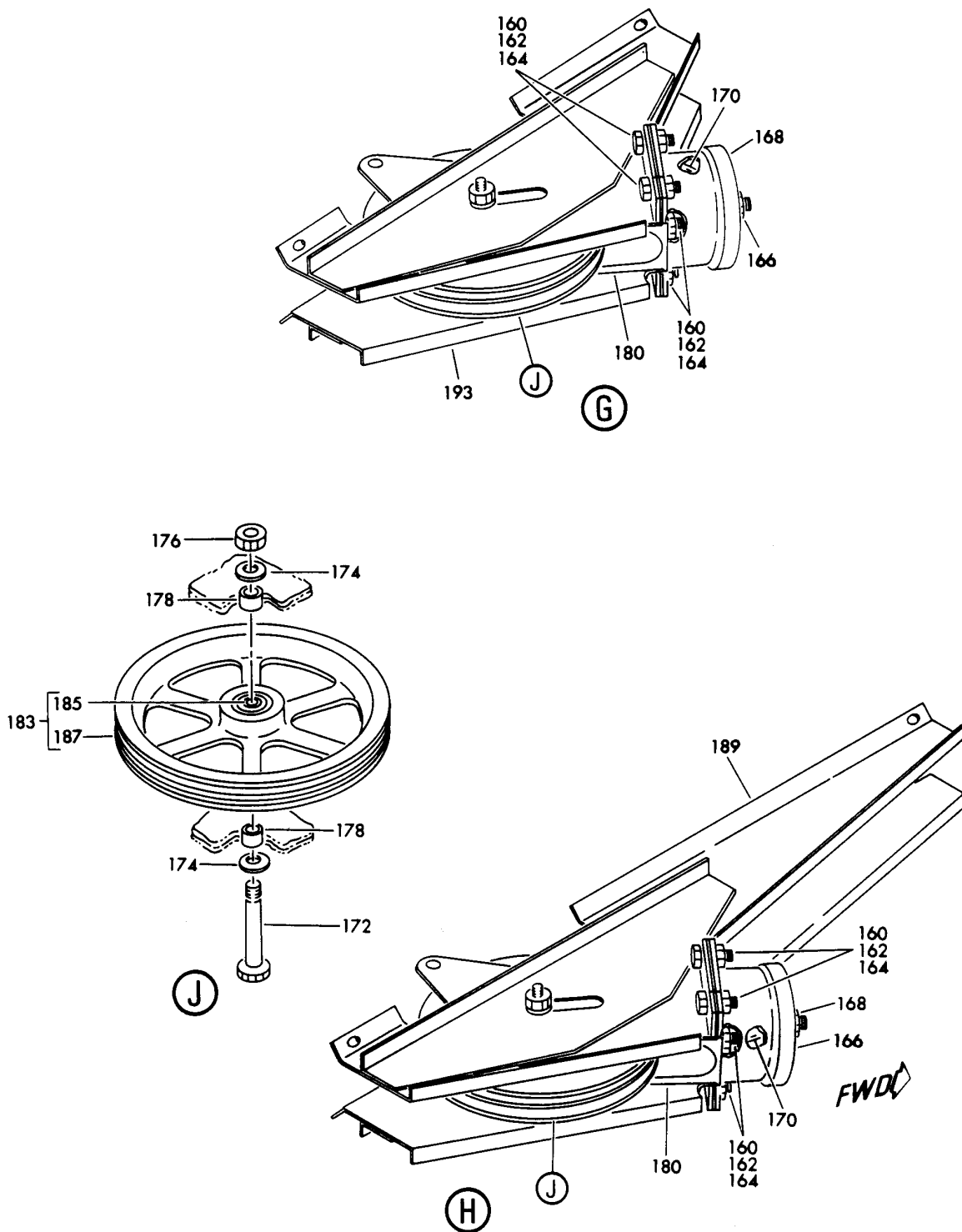
COUNTERBALANCE AND PULLEY INSTL-ENTRY AND SERVICE DOORS, SECT. 46 FIGURE 2 (SHEET 3)
