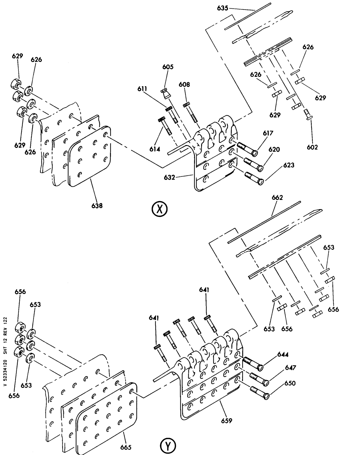
STRUCTURE ASSY-LARGE CARGO DOOR FIGURE 20 (SHEET 12)
