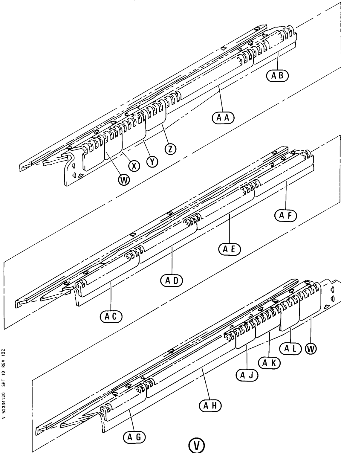
STRUCTURE ASSY-LARGE CARGO DOOR FIGURE 20 (SHEET 10)
