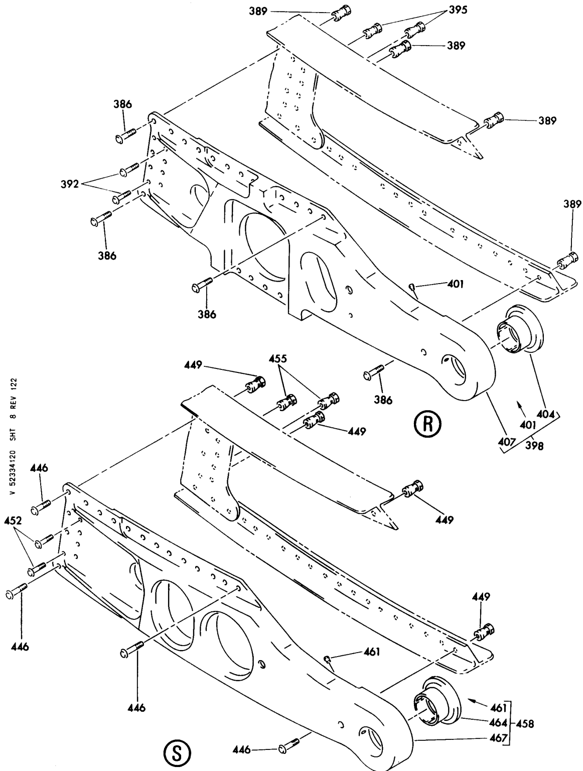
STRUCTURE ASSY-LARGE CARGO DOOR FIGURE 20 (SHEET 8)
