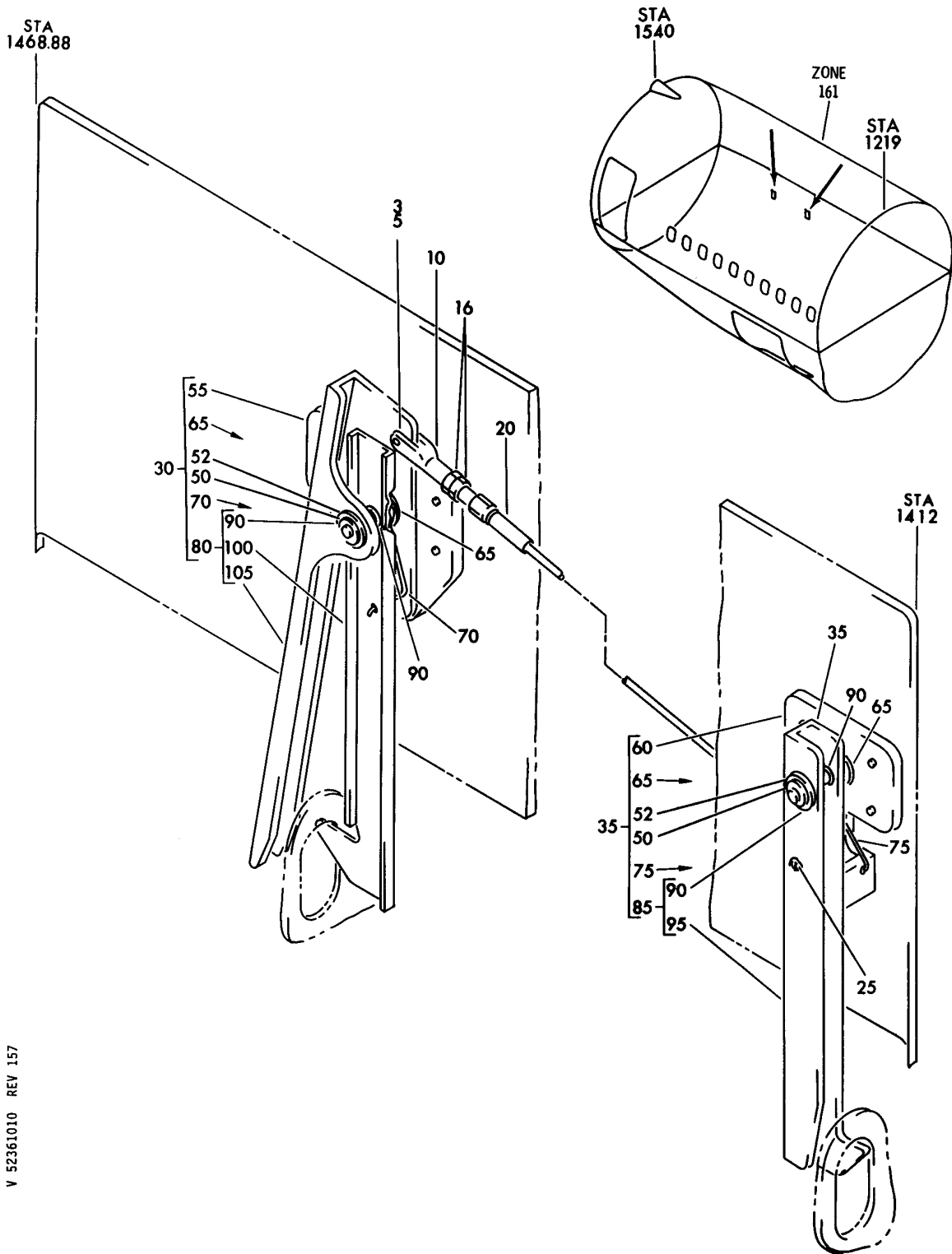
LATCH INSTL-SECT. 46 BULK CARGO DOOR PROTECTOR UP FIGURE 10
