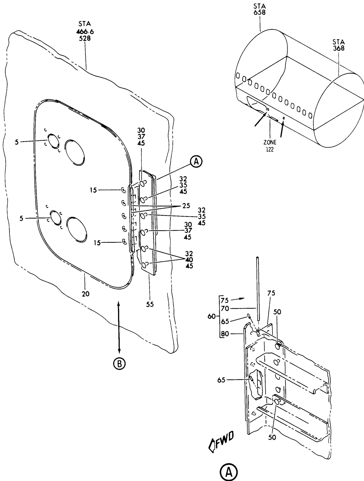
PAN AND DOOR INSTL-CARGO LOADING CONT FIGURE 1 (SHEET 1)
