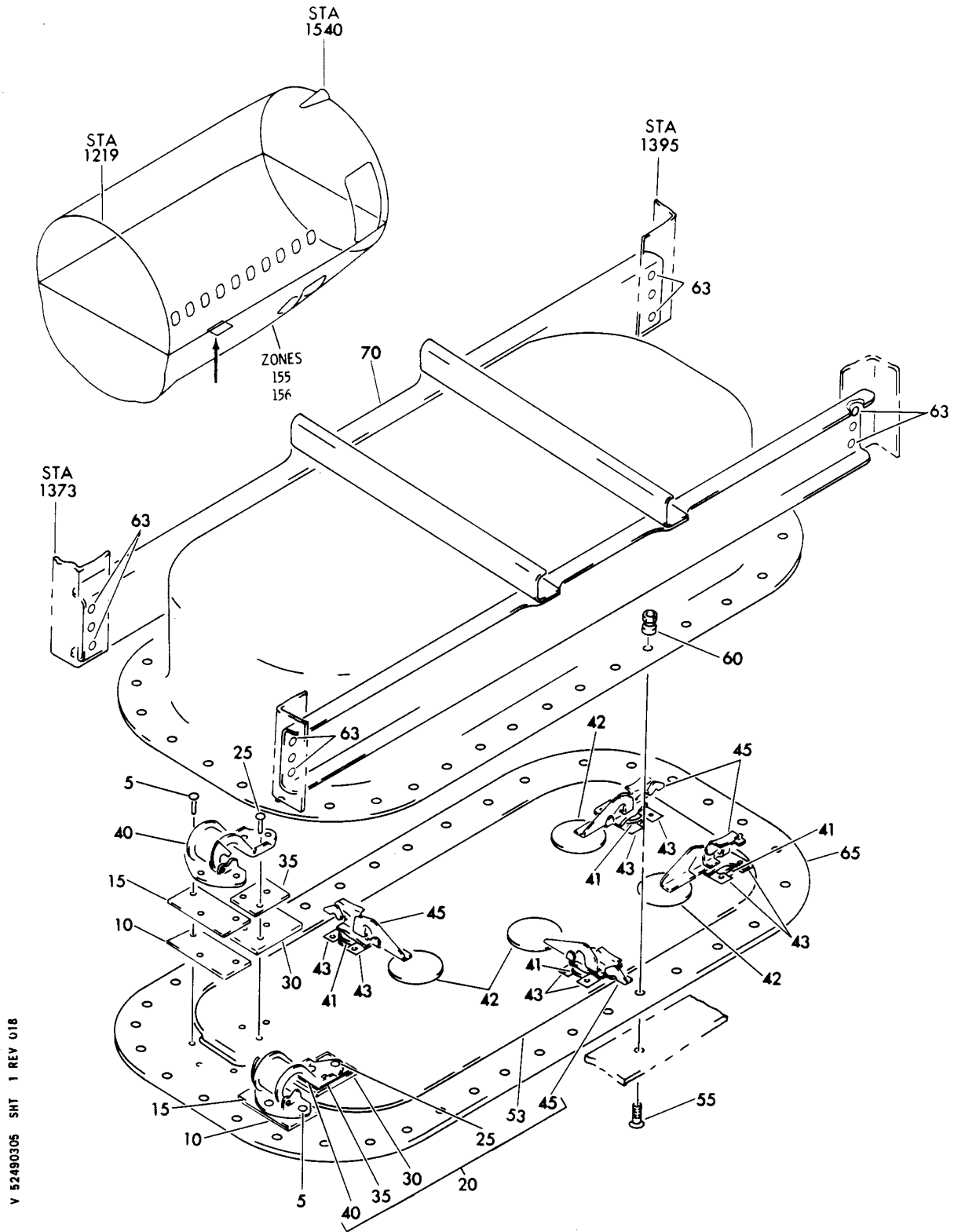
PAN AND DOOR INSTL-SECT. 46 POTABLE WATER SVCE FIGURE 5
