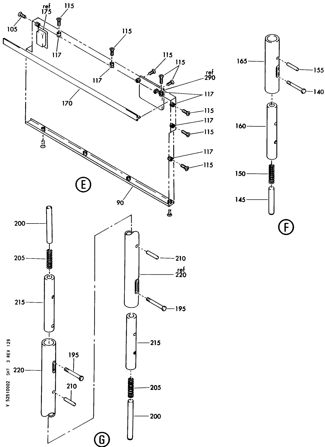
DOOR INSTL-FLIGHT DECK FIGURE 2 (SHEET 3)
