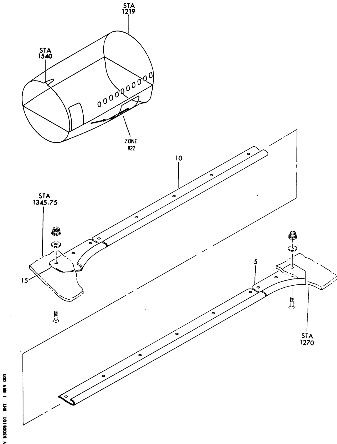
PLATE INSTL-CARGO SCUFF AFT FIGURE 1
