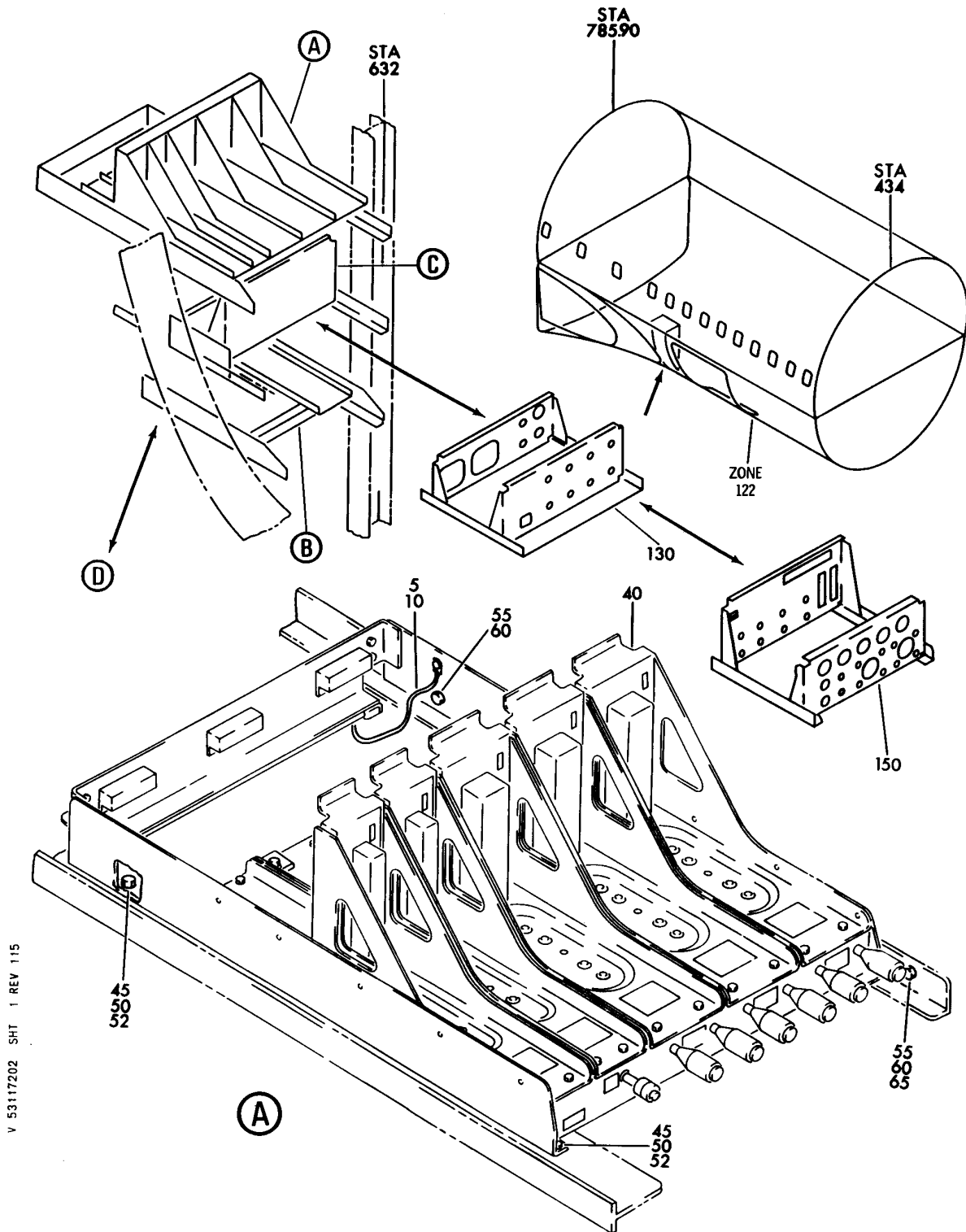
SHELF INSTL-ELECTRONICS EQPT CTR E5 RACK (CARGO DOOR) FIGURE 2 (SHEET 1)
