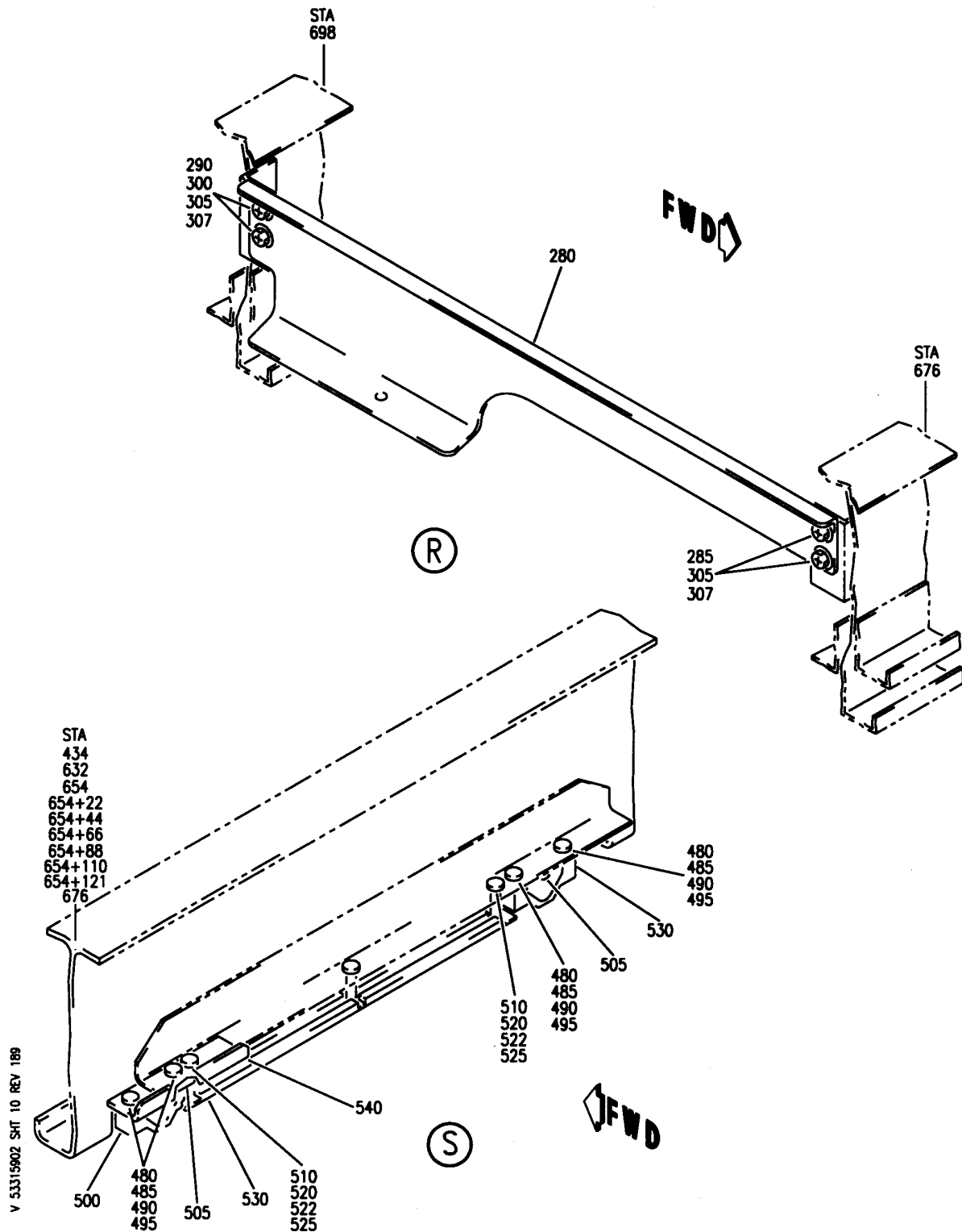
PROVISION INSTL-SECT. 43 LWR WIRE FIGURE 2 (SHEET 10)
