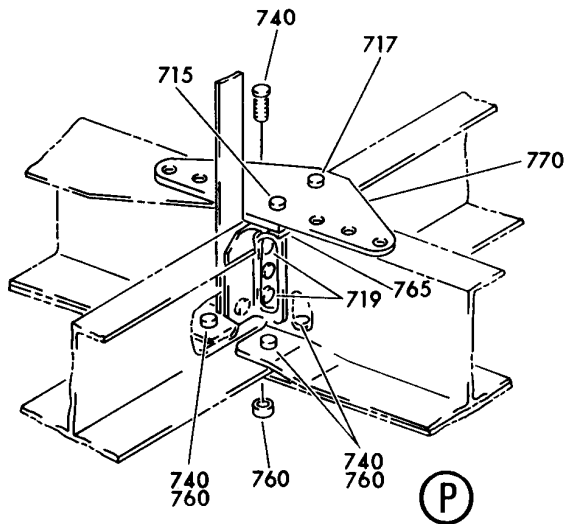
STRUCTURE ASSY-UNDERWING FAIRING SPRT FIGURE 1 (SHEET 7)
