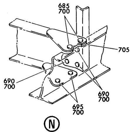
STRUCTURE ASSY-UNDERWING FAIRING SPRT FIGURE 1 (SHEET 7)
