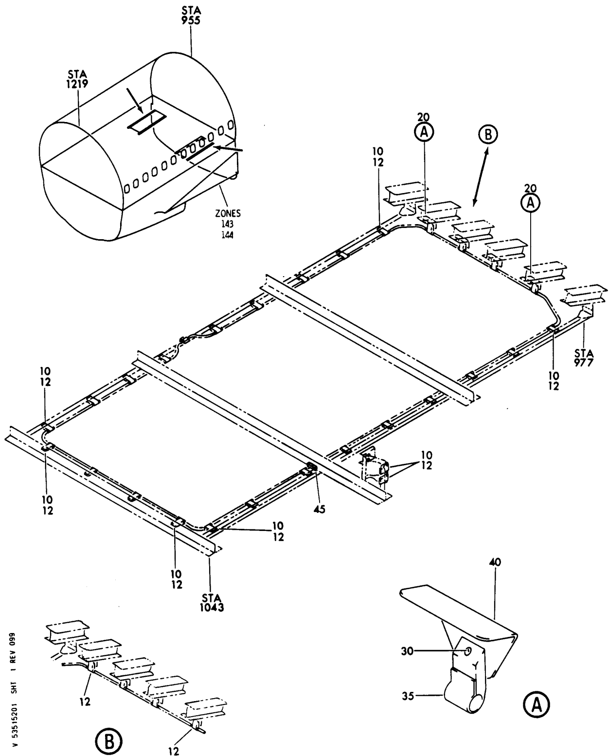
SUPPORT INSTL-MAIN WHL WELL OVERHEAT FIGURE 1
