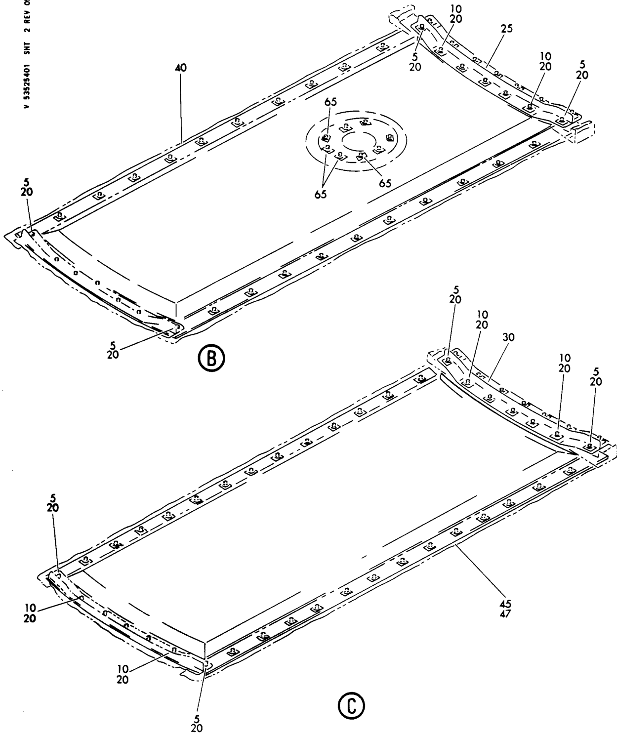
PANEL INSTL-KEEL BEAM FAIRING FIGURE 1 (SHEET 2)
