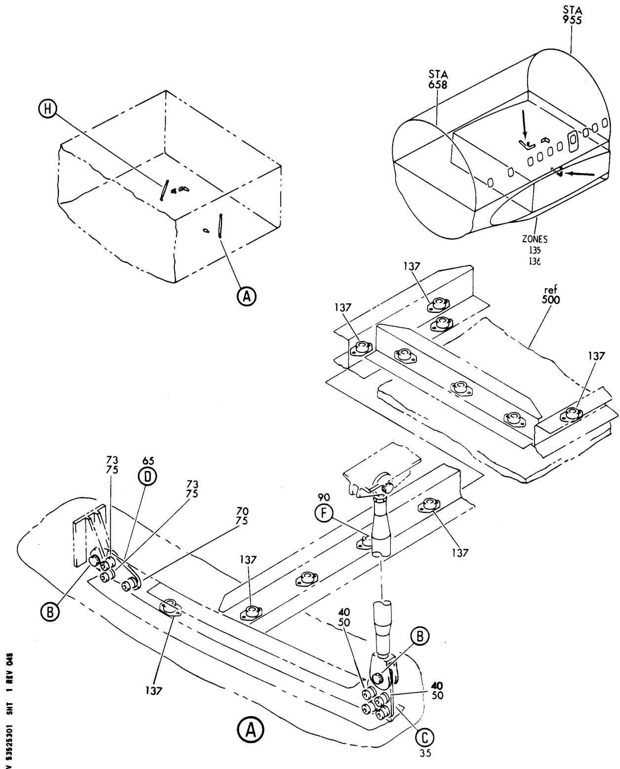
FRAME ASSY-UNDERWING FARING ENVIRONMENTAL CONT SYS EXH FIGURE 1 (SHEET 1)
