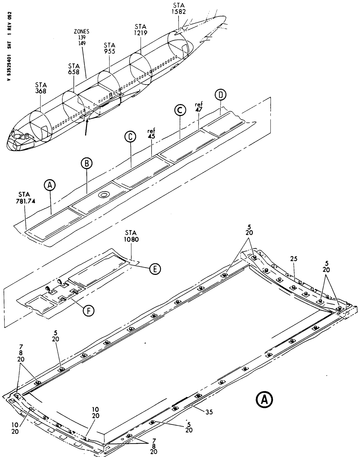
PANEL INSTL-KEEL BEAM FAIRING FIGURE 1 (SHEET 1)
