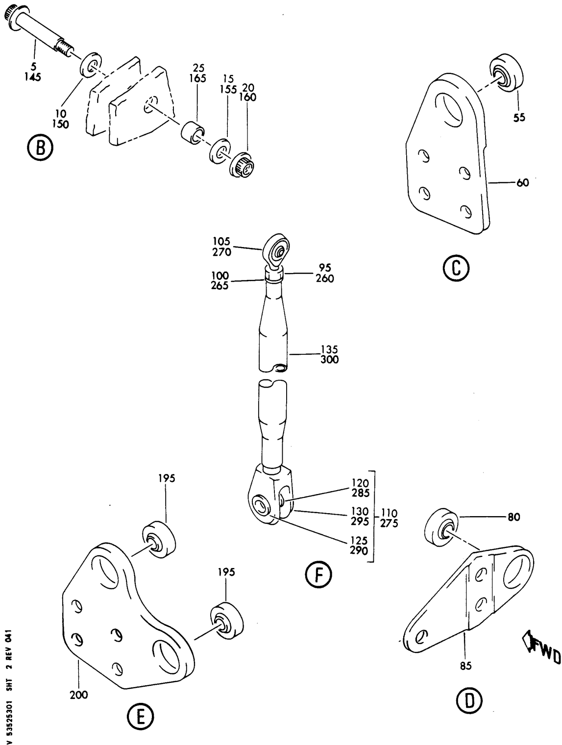
FRAME ASSY-UNDERWING FARING ENVIRONMENTAL CONT SYS EXH FIGURE 1 (SHEET 2)
