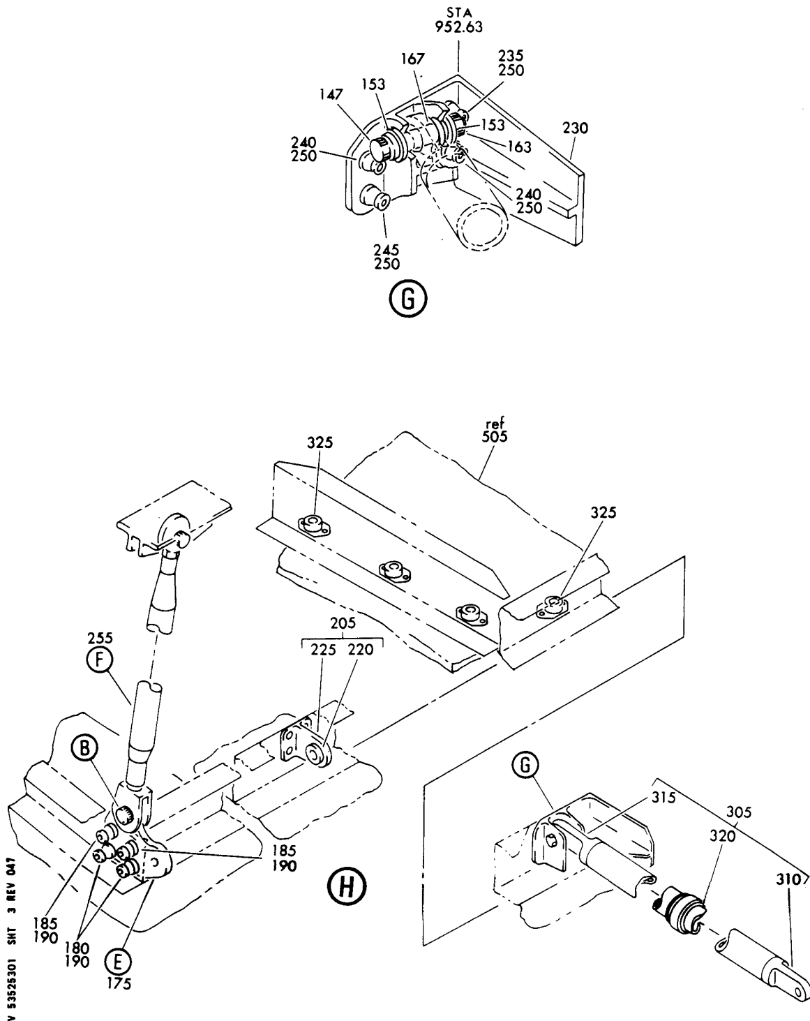
FRAME ASSY-UNDERWING FARING ENVIRONMENTAL CONT SYS EXH FIGURE 1 (SHEET 3)
