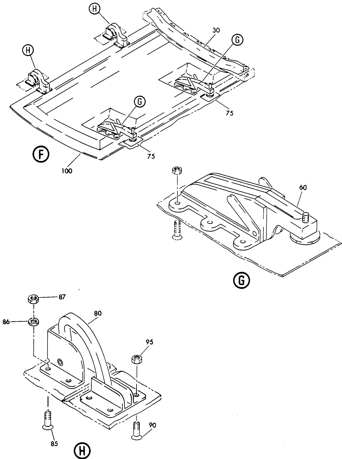
PANEL INSTL-KEEL BEAM FAIRING FIGURE 1 (SHEET 4)
