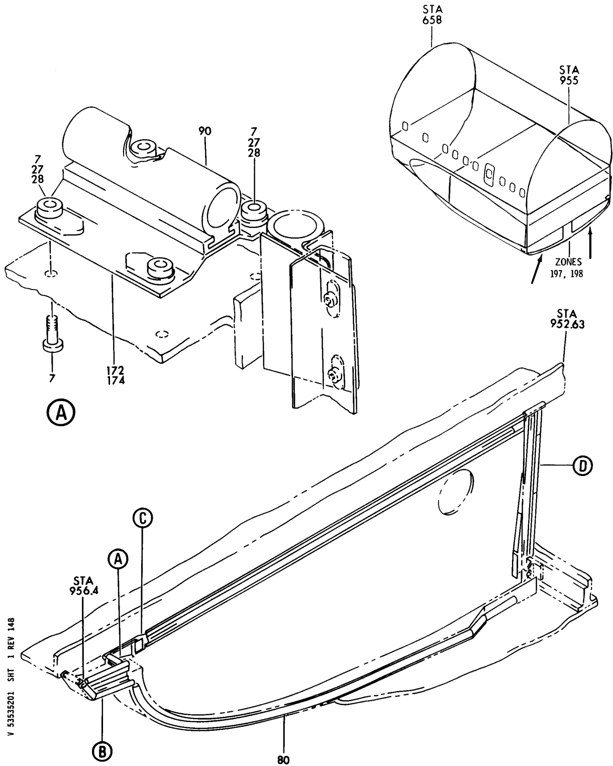
SEAL INSTL-UNDERWING FAIRING VAPOR BARRIER FIGURE 1 (SHEET 1)
