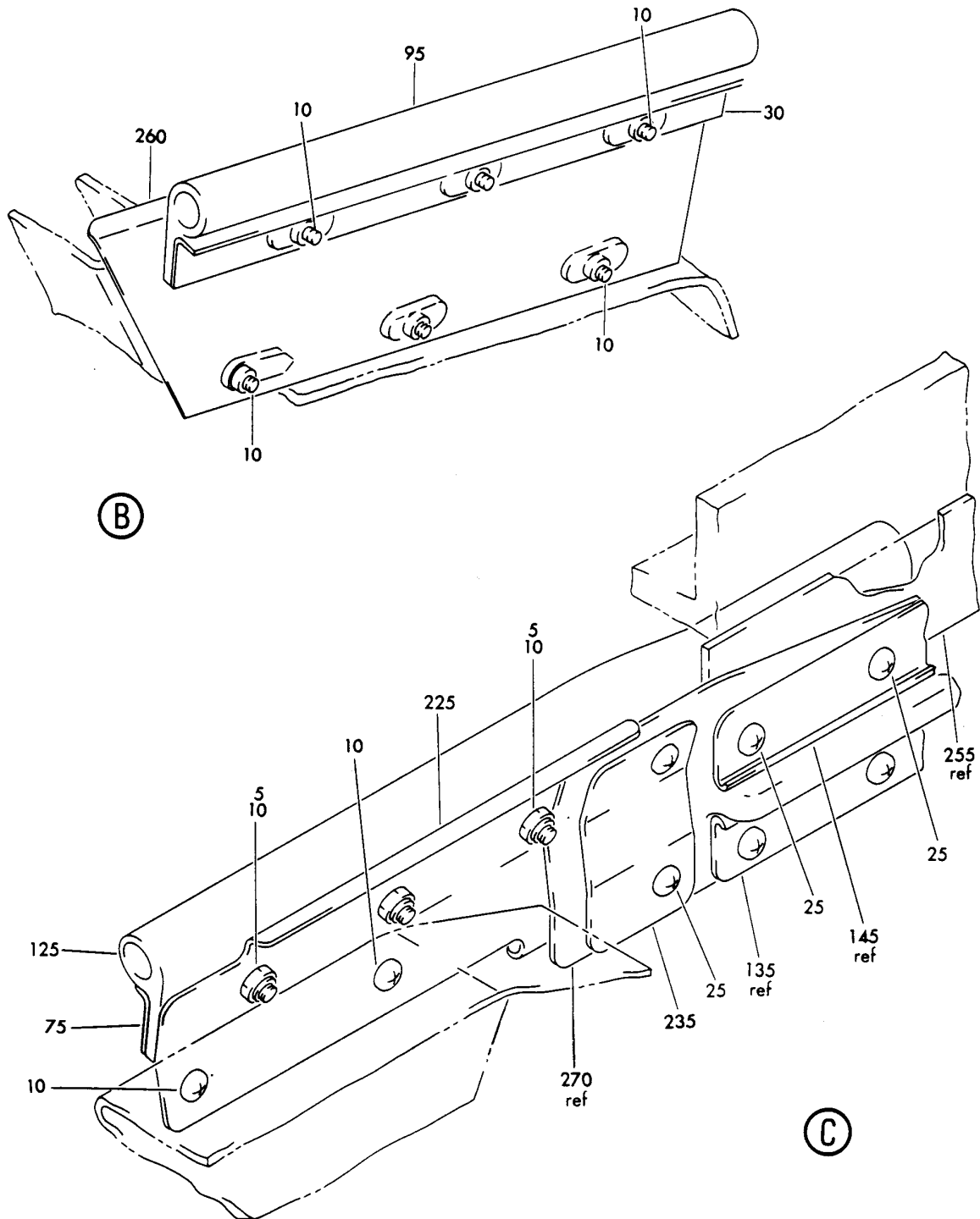
SEAL INSTL-UNDERWING FAIRING VAPOR BARRIER FIGURE 1 (SHEET 2)
