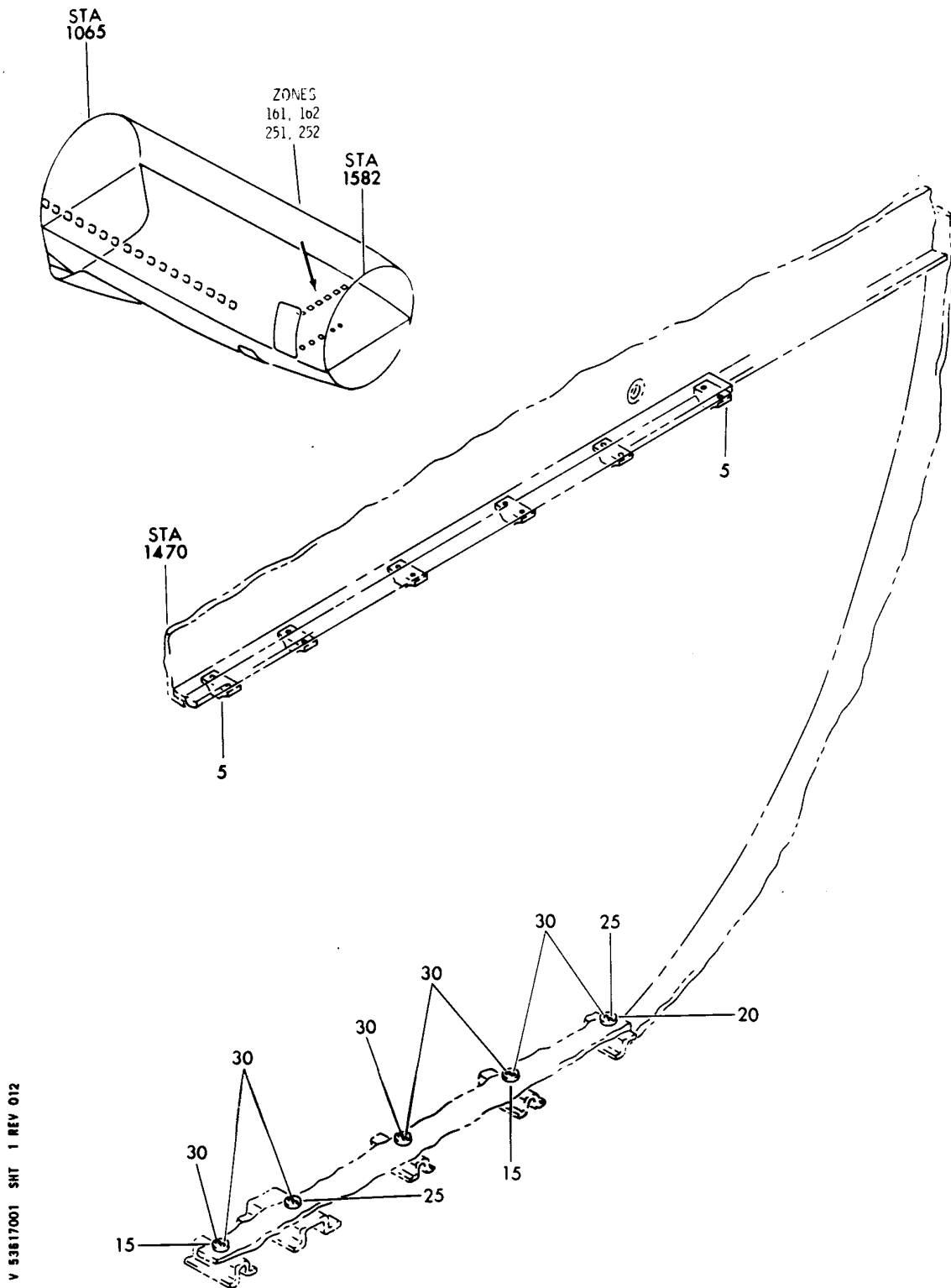
FITTING INSTL-TRANSVERSE NET FIGURE 1
