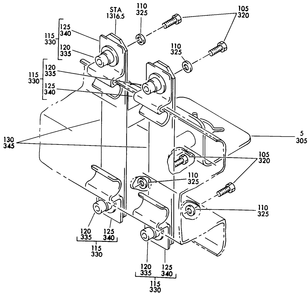
BRACKET INSTL-SECT. 46 VHF ANT. C WIRE PROVISION DISC. LWR FIGURE 1
