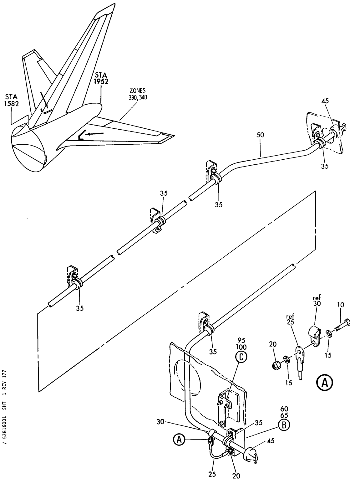
PROVISION INSTL-HORIZ STAB. WIRE VAR FIGURE 1 (SHEET 1)
