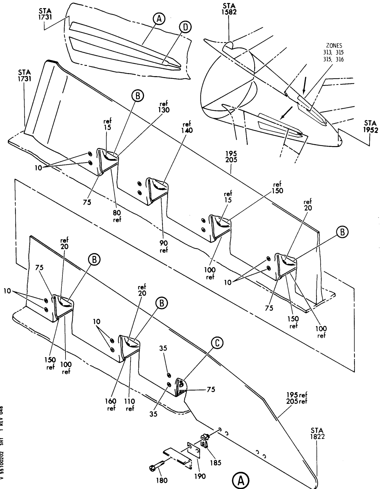
SEAL INSTL-HORIZ STAB. TO BODY FIGURE 2 (SHEET 1)
